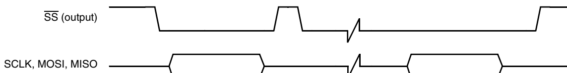
Figure 16. Master SPI Timing Diagram Ignore \overline{\text{SPI\_RDY}} Level Trigger
