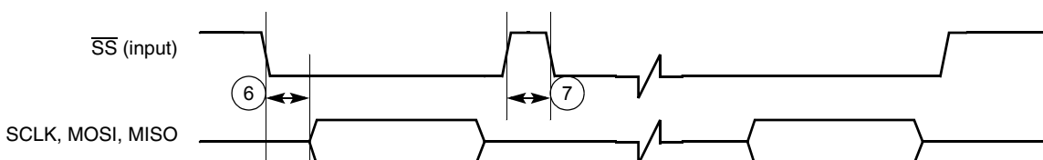
Figure 18. Slave SPI Timing Diagram FIFO Advanced by \overline{\text{SS}} Rising Edge
