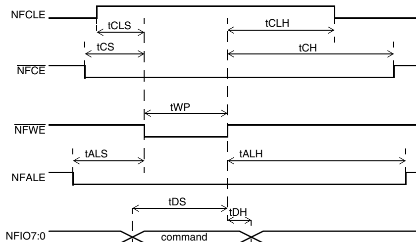
Figure 33. Command Latch Cycle Timing
