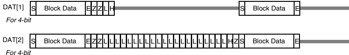
Figure 32. SDIO ReadWait Timing Diagram
