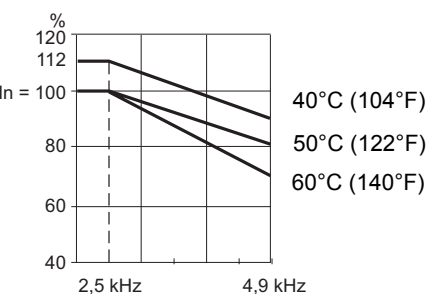
ATV71HC25Y
