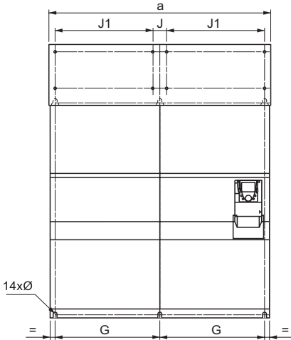
ATV71HC40Y 至 C63Y
