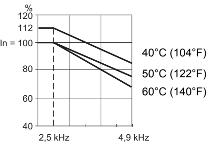
ATV71HC50Y
