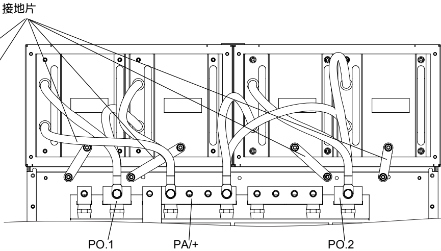
示例 4: ATV71H C40N4 ... C50N4
