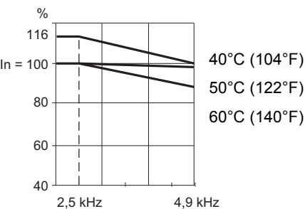
ATV71HC40Y
