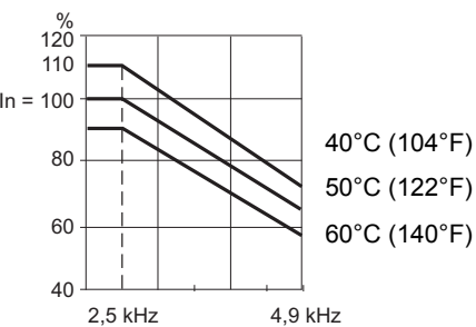
ATV71HC16Y
