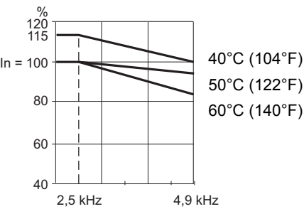
ATV71HC11Y
