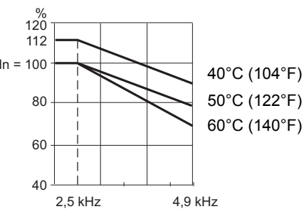
ATV71HC13Y
