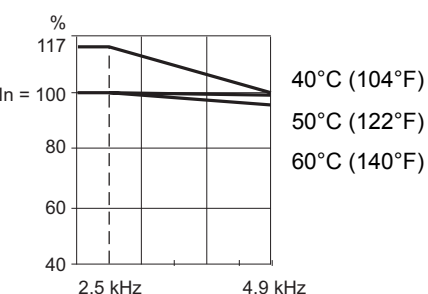
ATV71HC20Y
