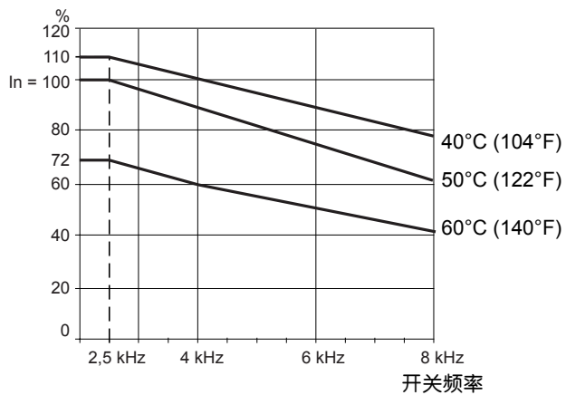
ATV71HC31N4
