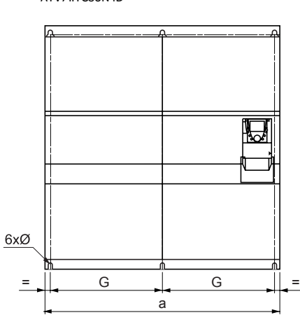
ATV71H C50N4D
