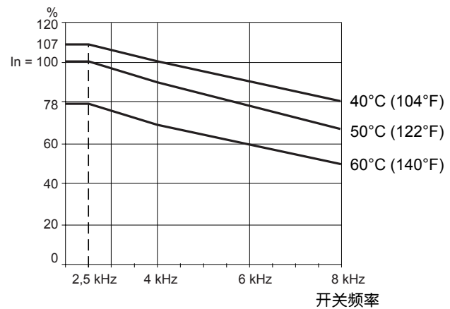
ATV71HC13N4
