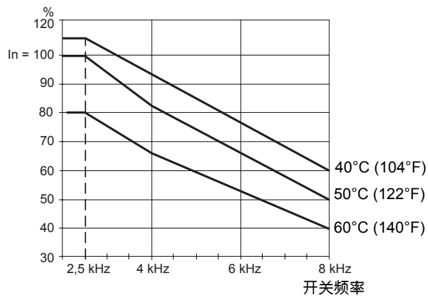
ATV71HC11N4
