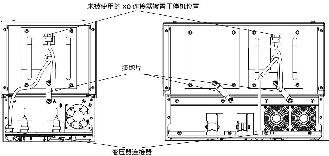
示例 3：ATV71H C40Y ... C63Y
