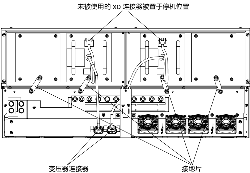
示例 3：ATV71H C40Y ... C63Y
