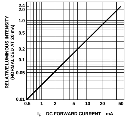
Figure 10. Relative Luminous Intensity vs. DC Forward Current.
