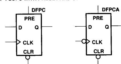
Figure 23. D-Type Flip-Flops
