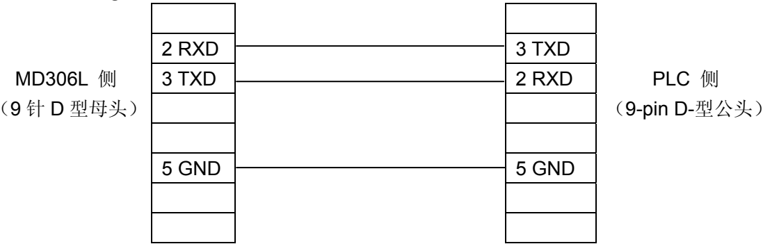
Connection guidance of MD2-LG-Mod cable
