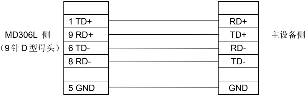
MD2-FREEPTC-RS422 连线图
