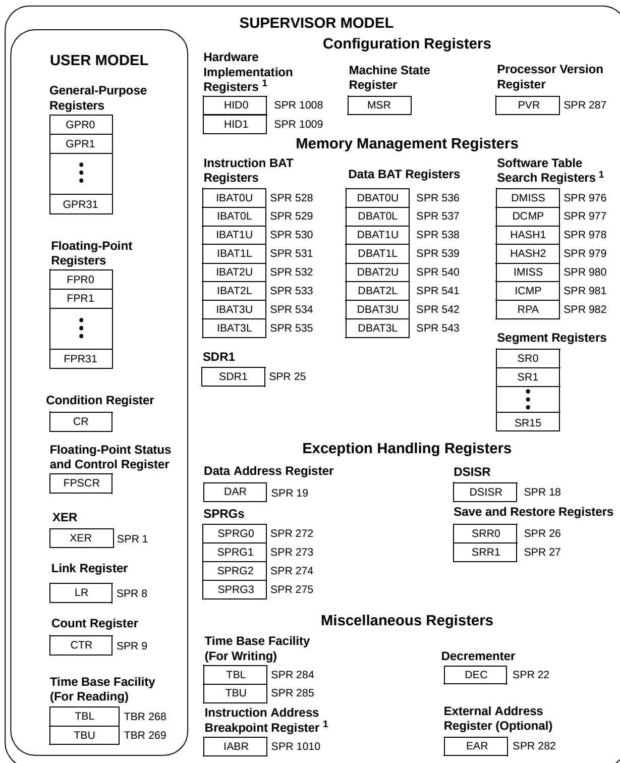
Figure 2-1. Programming Model—Registers
