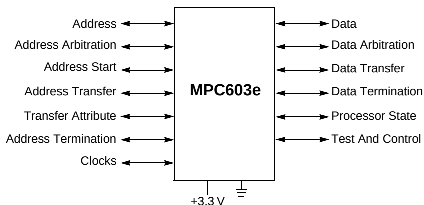
Figure 1-4. System Interface
