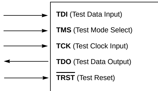
Figure 7-2. IEEE 1149.1-Compliant Boundary Scan Interface
