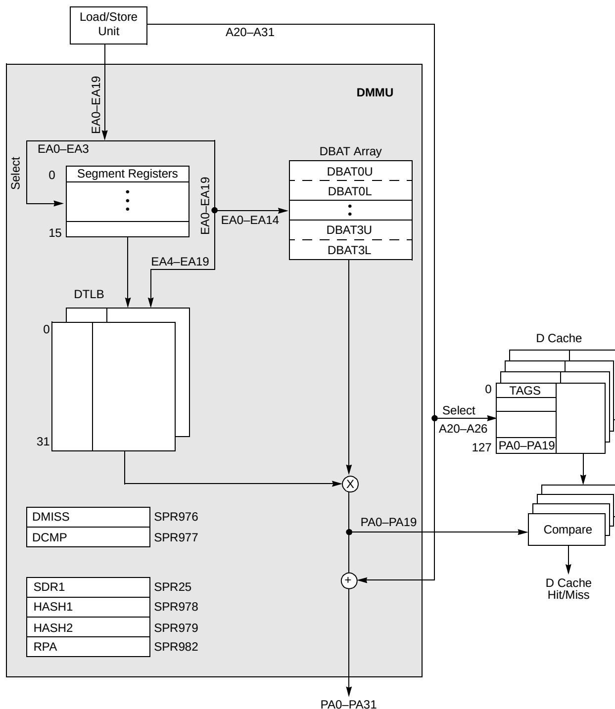
Figure 5-3. DMMU Block Diagram
