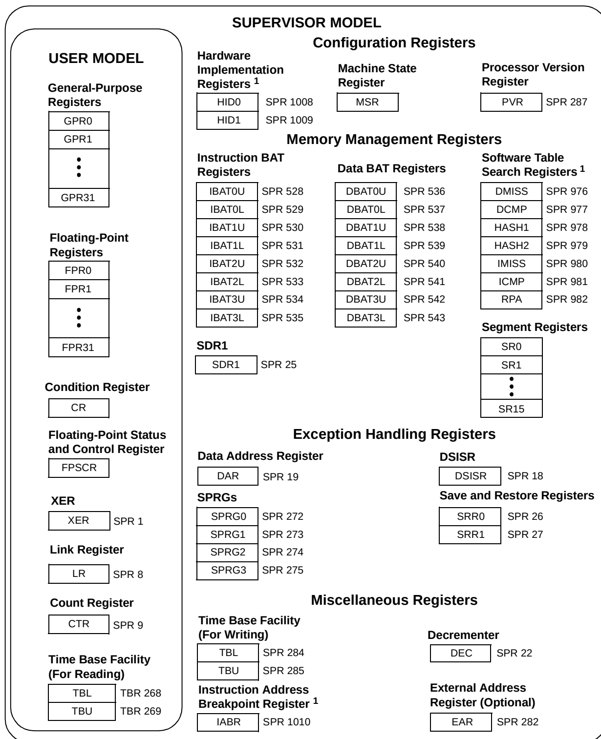
Figure 1-2. Programming Model—Registers
