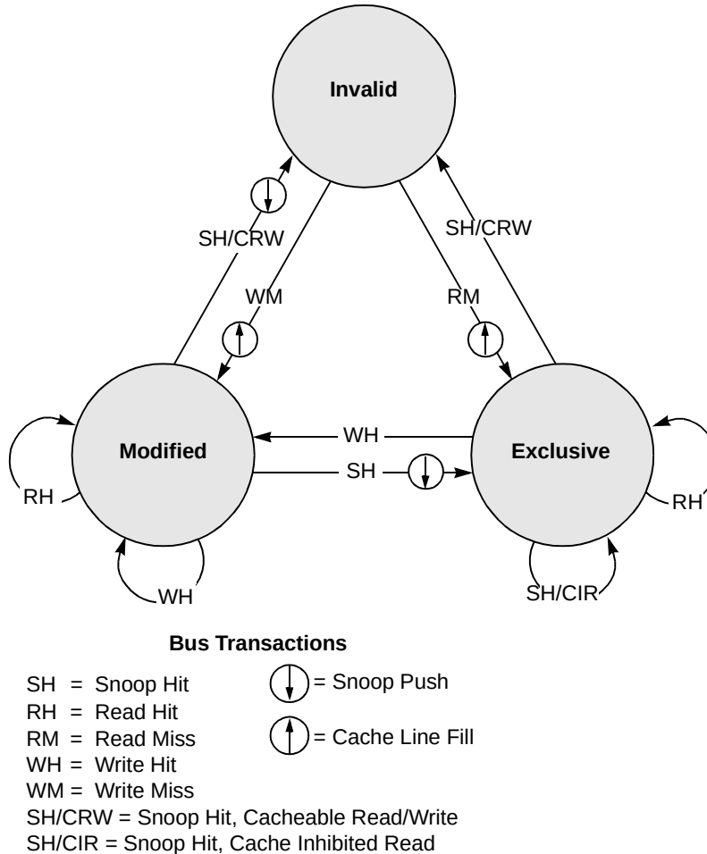
Figure 3-4. MEI Cache Coherency Protocol—State Diagram (WIM = 001)
