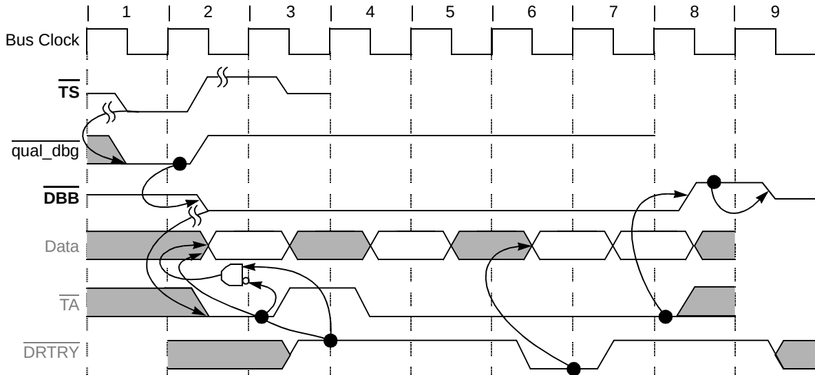
Figure 8-12. Read Burst with \overline{\text{TA}} Wait States and \overline{\text{DRTRY}}
