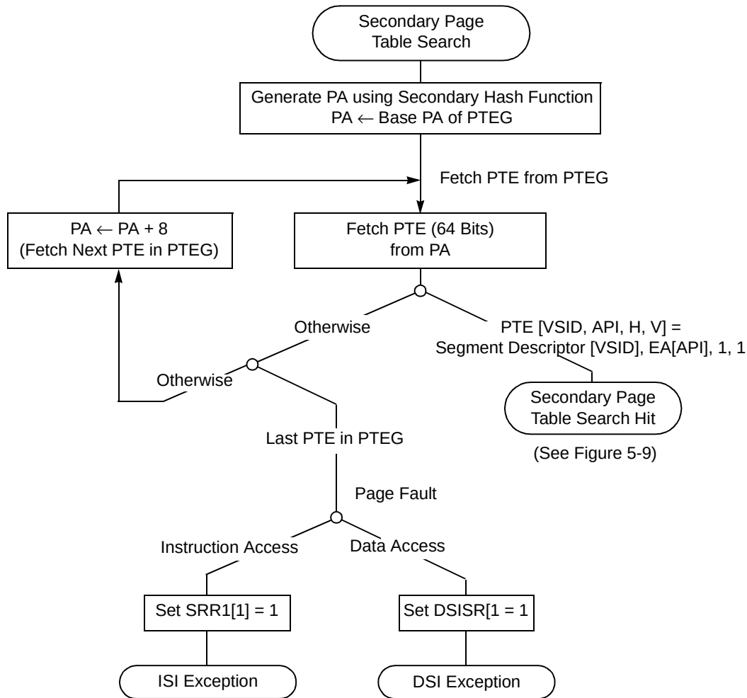
Figure 5-10. Secondary Page Table Search Flow—Conceptual Flow
