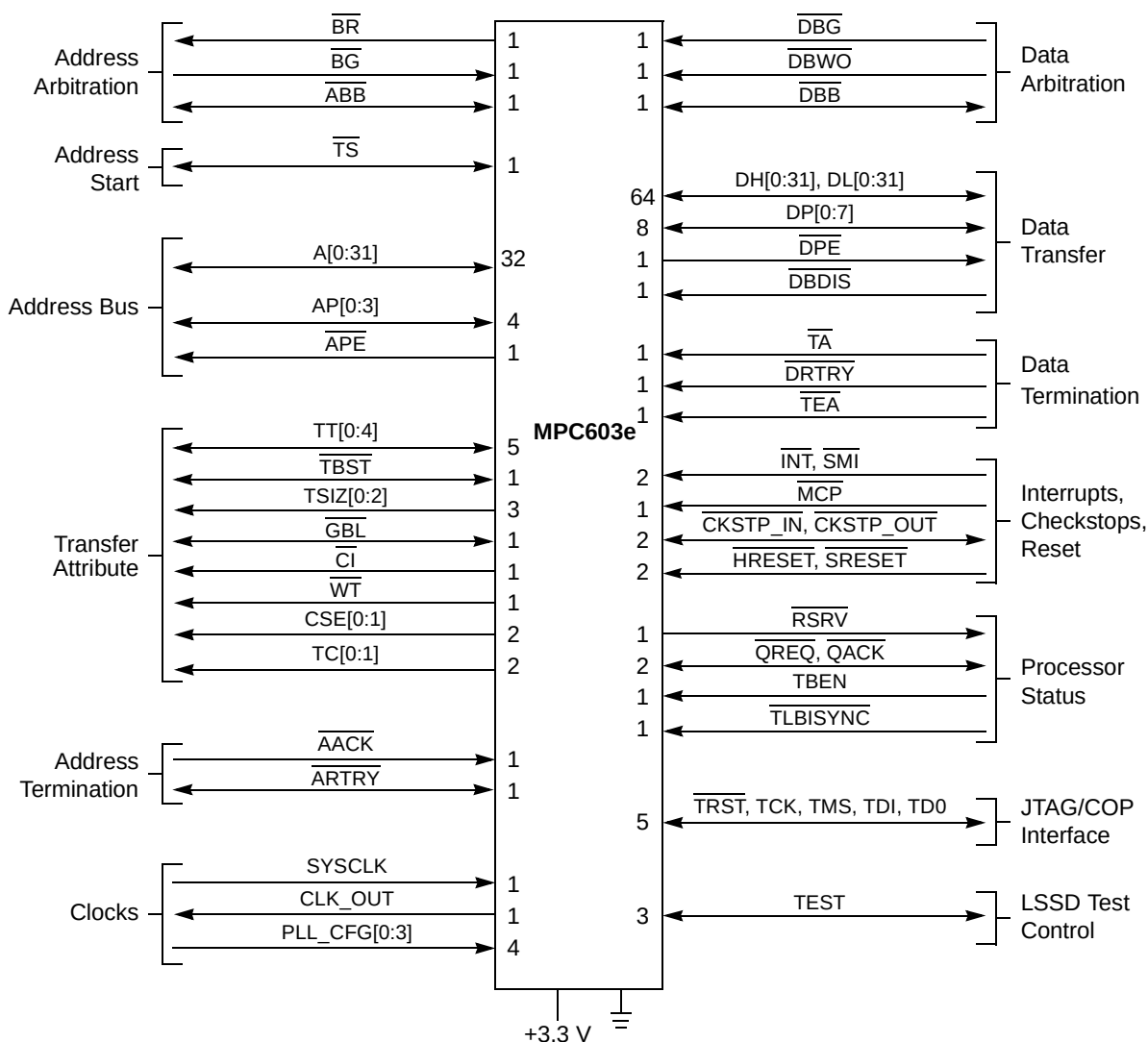
Figure 1-5. Signal Groups
