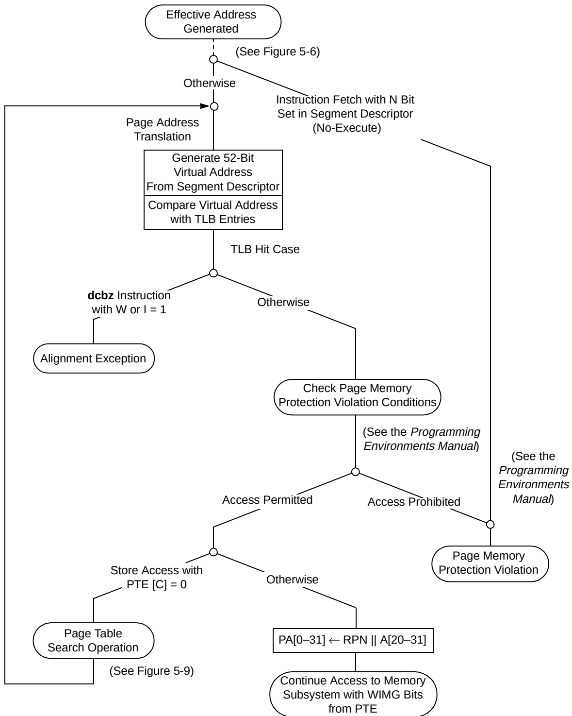
Figure 5-8. Page Address Translation Flow for 32-Bit Implementations—TLB Hit
