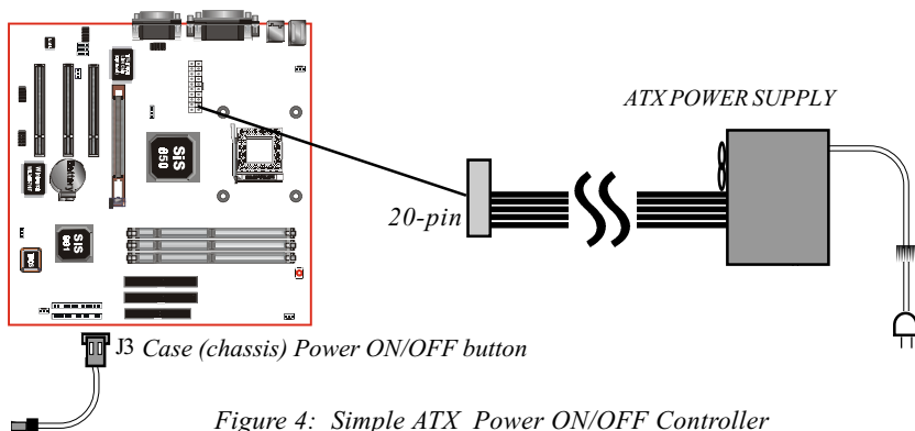
Figure 4: Simple ATX Power ON/OFF Controller
