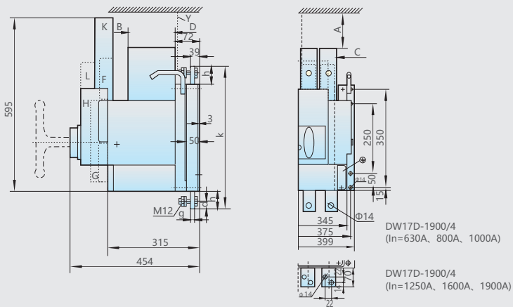
图16-2 DW17D-1900/4(In=630~1900)四极固定式垂直接线
