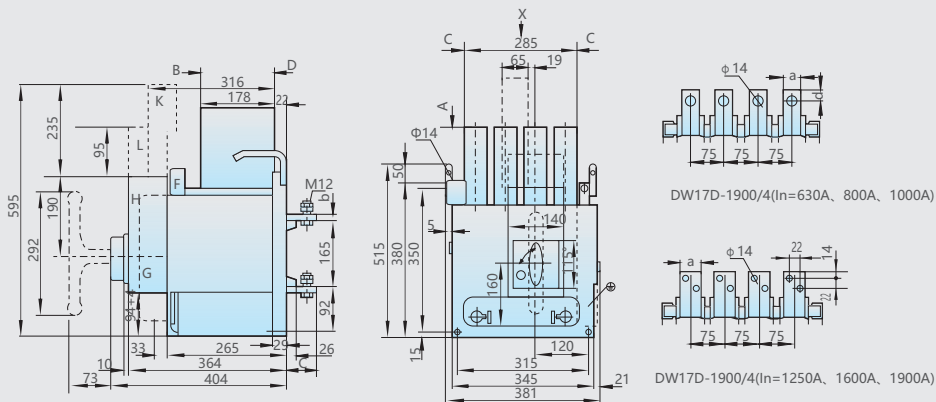
图16-1 DW17D-1900/4(In=630~1900)四极固定式水平接线
