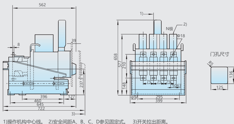
图16-5 DW17D-1900/4(In=630A~1600A)四极抽屉式接线
