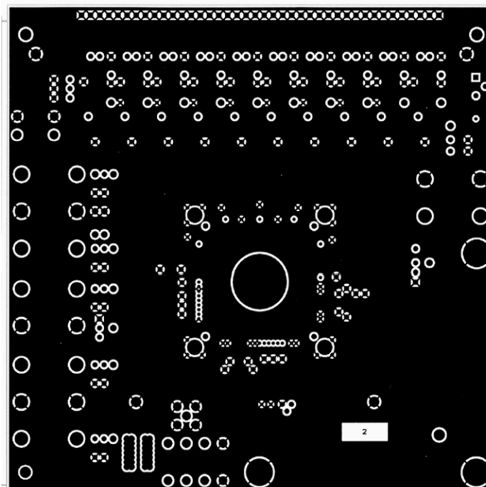
Figure 6-9. Ground Plane
