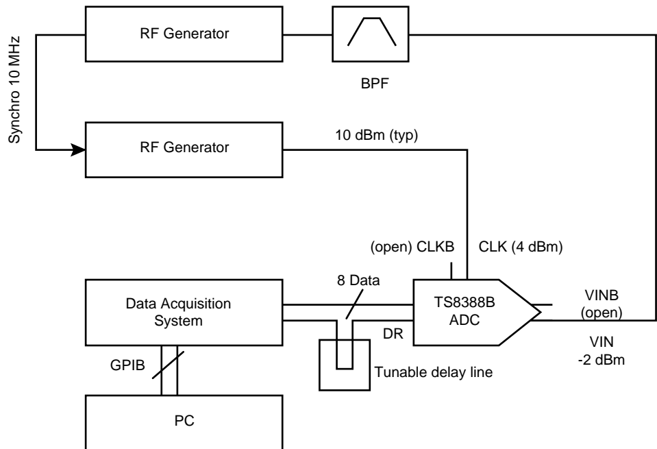
Figure 4-5. Single-ended Analog and Clock Input Configuration
