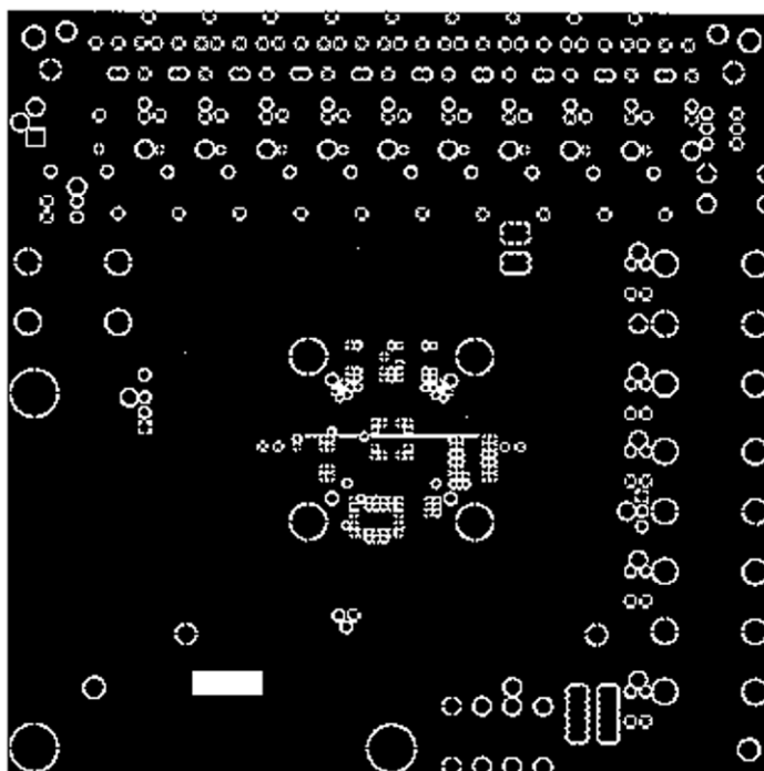
Figure 6-5. Ground Plane
