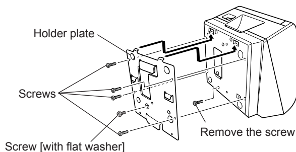
fig 1. Attaching the holder plate
