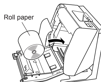
fig 4. Setting the roll paper in place
