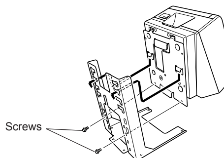
fig 3. Setting the printer on the stand
