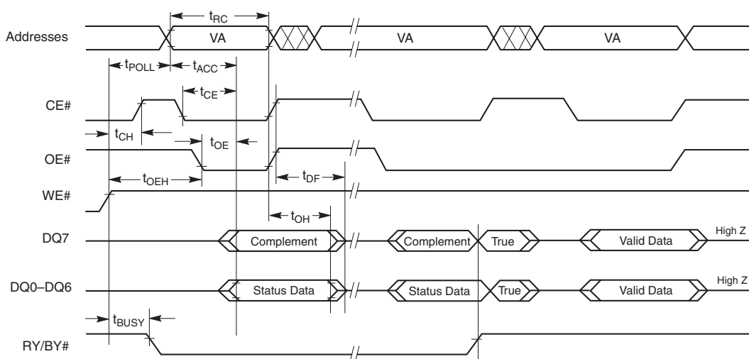
Figure I8. Chip/Sector Erase Operation Timings
