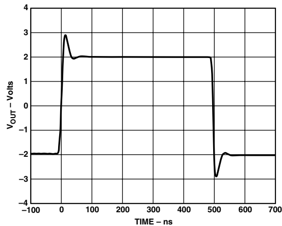
TPC 3. 4 V Step Response; G = +5 , V_S = \pm 6\text{ V} , R_L = 25\ \Omega , Single-Ended
