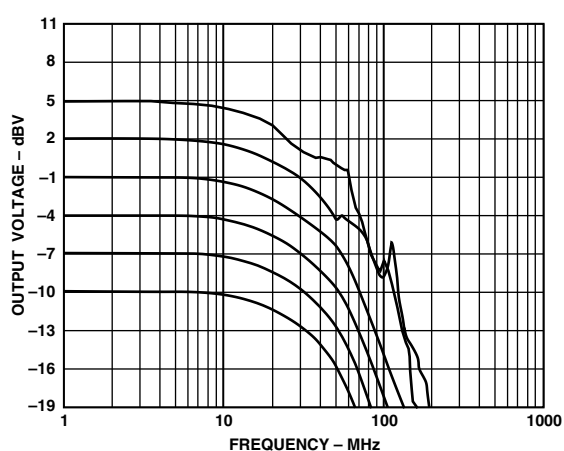
TPC 18. Output Voltage vs. Frequency; V_S = \pm 6 V, R_L = 100 \Omega ; G = +5
