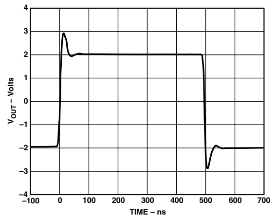
TPC 6. 4 V Step Response; G = +5 , V_S = \pm 12\text{ V} , R_L = 100\ \Omega , Single-Ended
