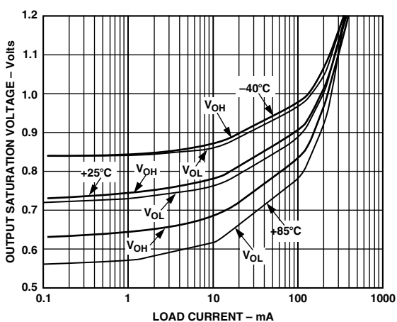
TPC 15. Output Saturation Voltage vs. Load; V_S = \pm 12 V, V_S = \pm 6 V
