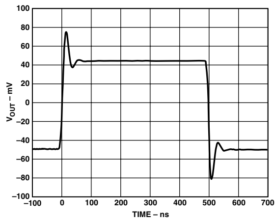
TPC 2. 100 mV Step Response; G = +5 , V_S = \pm 6\text{ V} , R_L = 25\ \Omega , Single-Ended
