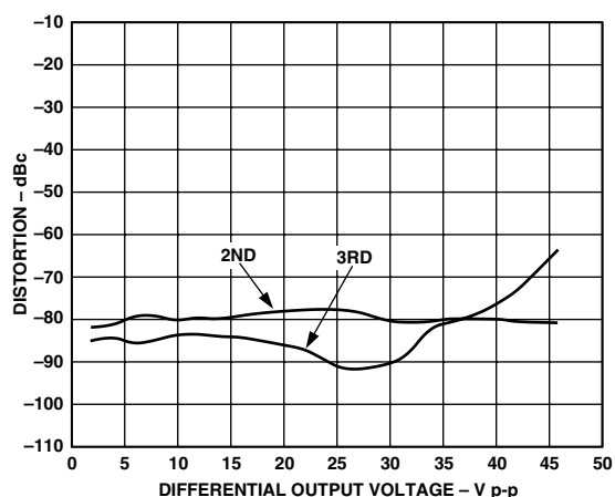
TPC 14. Distortion vs. Output Voltage; f = 500 kHz, V_S = \pm 12 V, G = +10 , R_L = 200 \Omega , Differential
