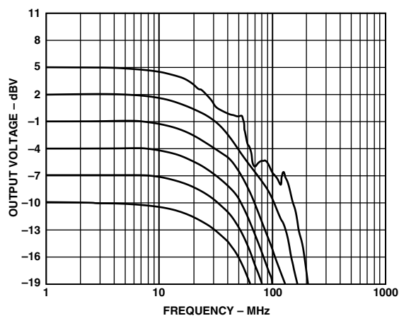
TPC 16. Output Voltage vs. Frequency; V_S = \pm 12 V, R_L = 100 \Omega ; G = +5
