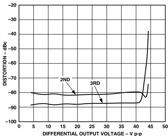
TPC 13. Distortion vs. Output Voltage; f = 100 kHz, V_S = \pm 12 V, G = +10 , R_L = 200 \Omega , Differential
