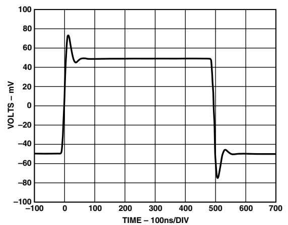
TPC 5. 100 mV Step Response; G = +5 , V_S = \pm 12\text{ V} , R_L = 100\ \Omega , Single-Ended
