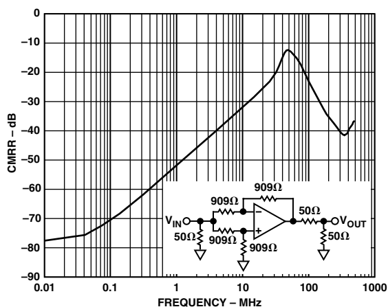
TPC 17. CMRR vs. Frequency; V_S = \pm 12 V, R_L = 100 \Omega
