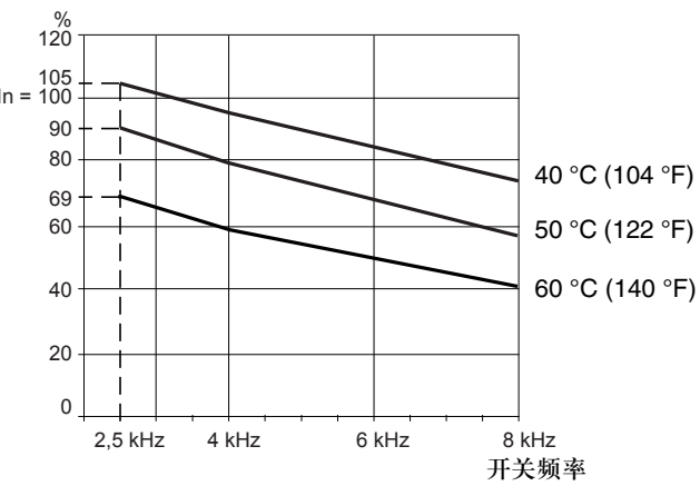
ATV61HC40N4
