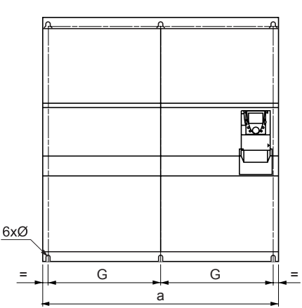
ATV61H C63N4D
