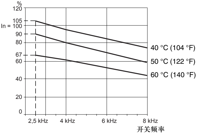
ATV61HC22N4
