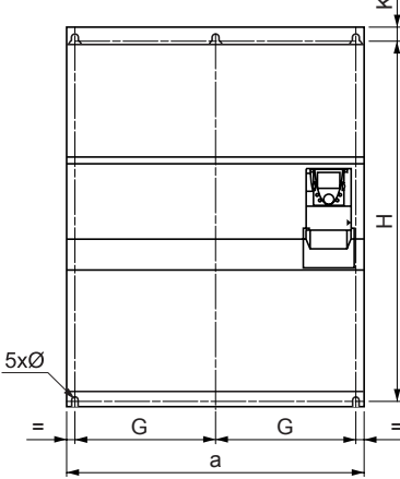
ATV61H C40N4D 至 C50N4D
