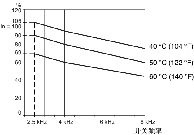
ATV61HC25N4
