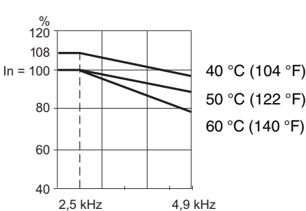
ATV61HC25Y
