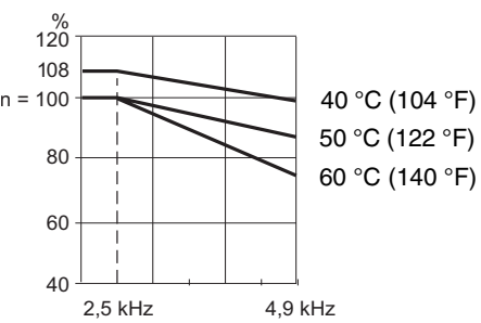
ATV61HC50Y
