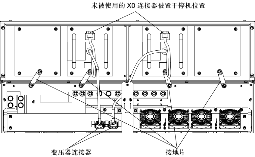
示例 3：ATV61H C50Y ... C80Y
