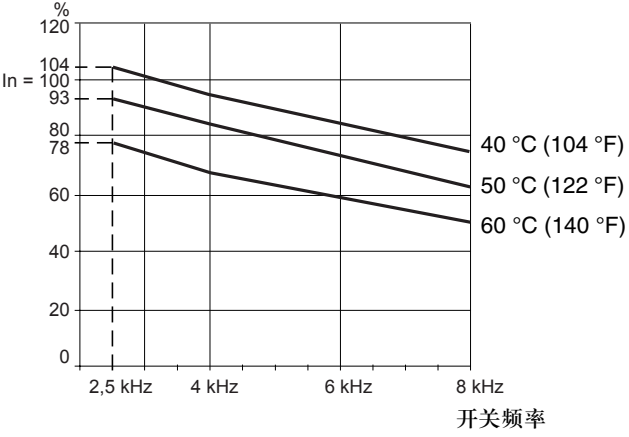
ATV61HC50N4
