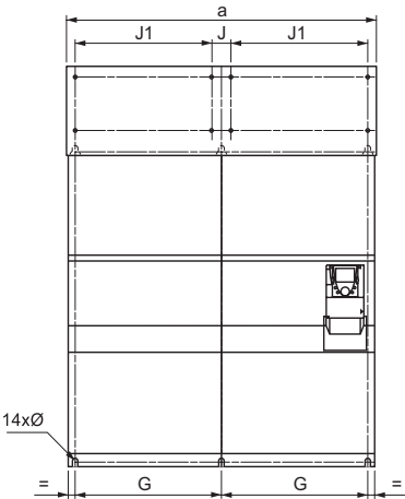
ATV61H C50Y 至 C80Y
