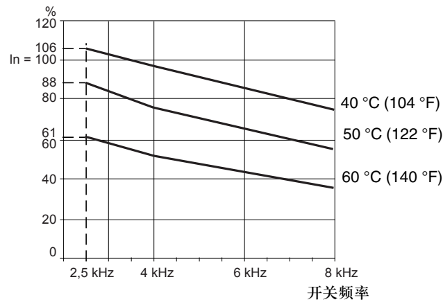
ATV61HC11N4
