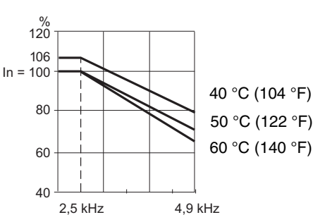
ATV61HC31Y
