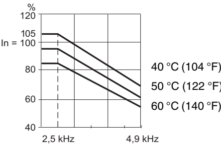
ATV61HC20Y
