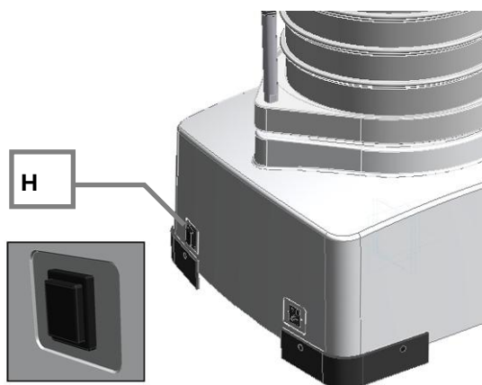
Fig. 10: Switching on/off
