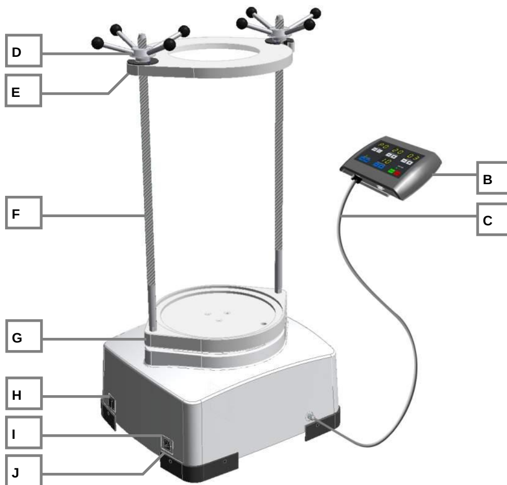
Fig. 4: Diagram of the components
