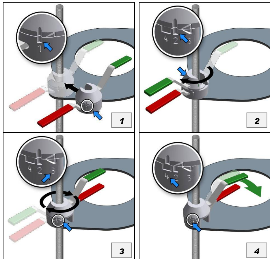
Fig. 9: Inserting and using the quick-action clamping device
