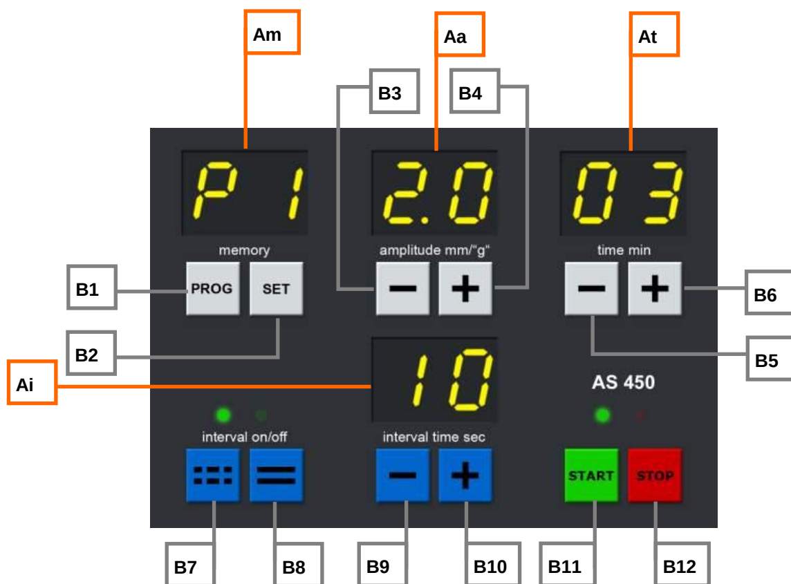
Fig. 6: Graphic Representation of the operating and display elements
