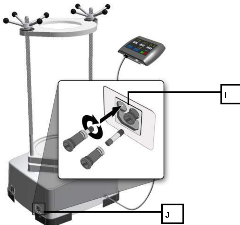
Fig. 20: Replacing the Fuses
