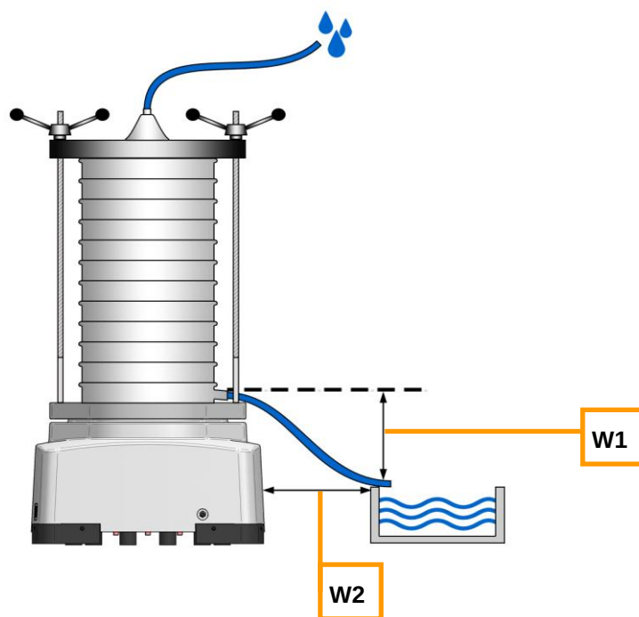
Fig. 17: Arrangement of the water system
