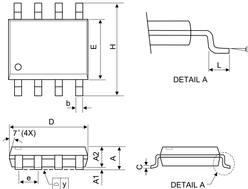
SOP-8L
