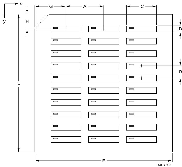
Fig.21 Tray details.
