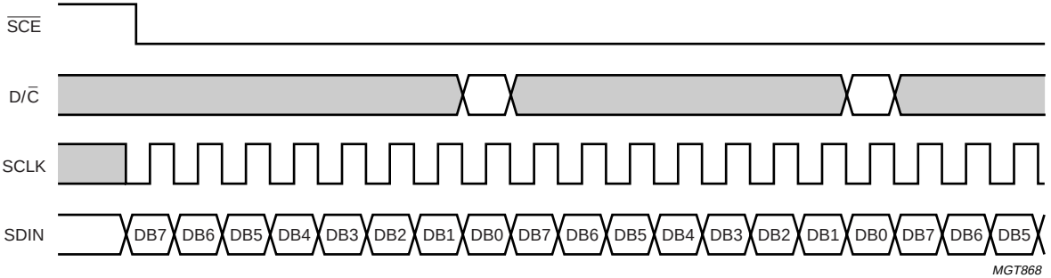
Fig.10 Serial bus protocol for transmission of several bytes.
