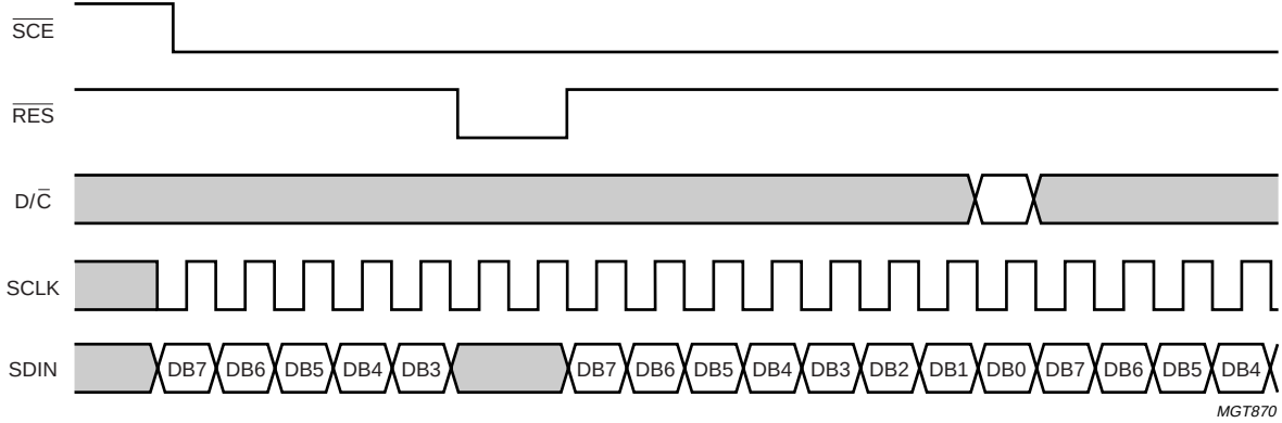
Fig.12 Serial bus interrupt function ( \overline{\text{RES}} ).
