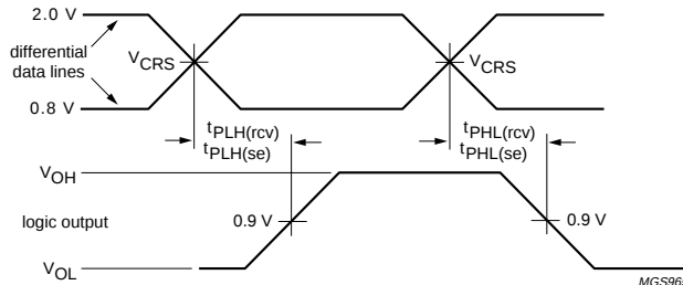
Fig 7. Timing of D+ and D– to RCV, VP and VM.
