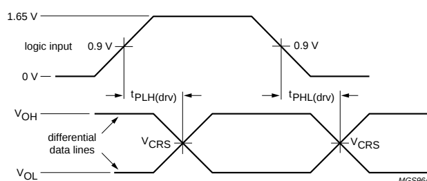
Fig 5. Timing of VPO/VO and VMO/FSE0 to D+ and D–.
