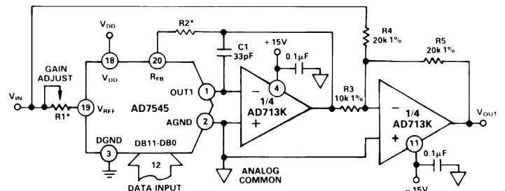
Figure 39. Bipolar Operation
