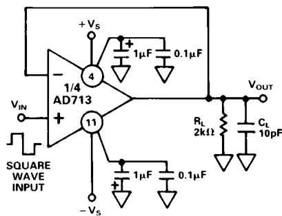
Figure 21a. Unity Gain Follower
