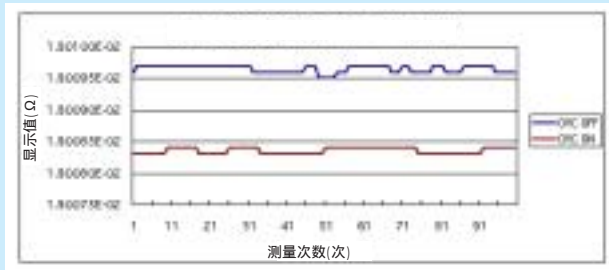
[20 mΩ 量程/慢2]
