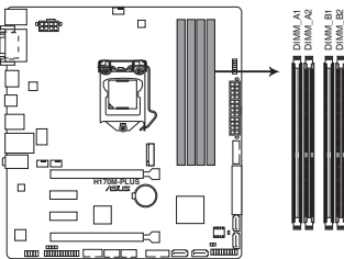
H170M-PLUS 288-pin DDR4 DIMM sockets
