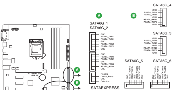
H170M-PLUS Intel® SATA 6.0Gb/s connectors
