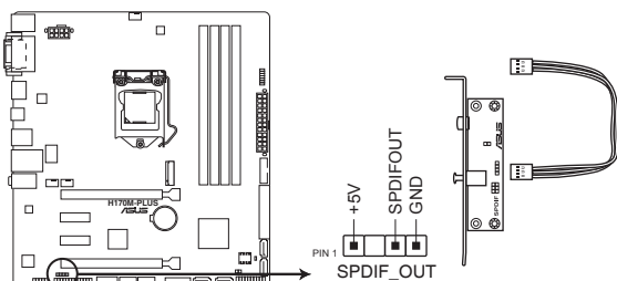
H170M-PLUS Digital audio connector
