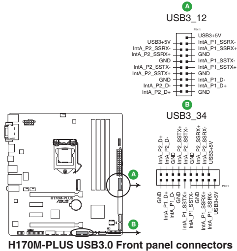
H170M-PLUS USB3.0 Front panel connectors
