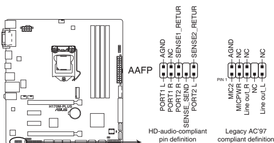
H170M-PLUS Front panel audio connector
