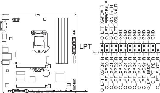
H170M-PLUS Parallel Port connector
