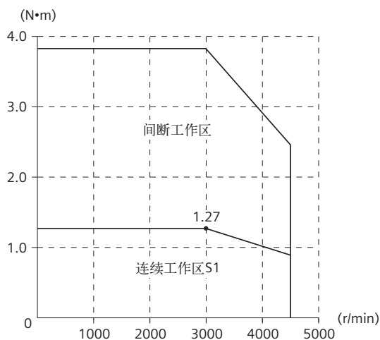
1FL4033-0AF21-.... (400W)
