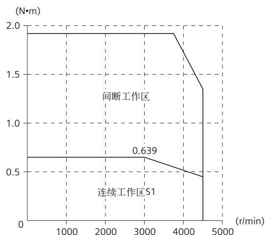
1FL4032-0AF32-.... (200W)
