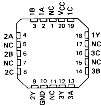
SN54LS10, SN54S10 . . . FK PACKAGE (TOP VIEW)
