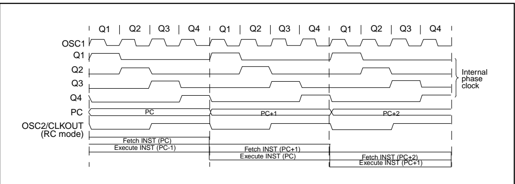
FIGURE 3-2: CLOCK/INSTRUCTION CYCLE
