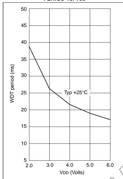
FIGURE 12-13: WDT TIMER TIME-OUT PERIOD vs. V_{DD}
