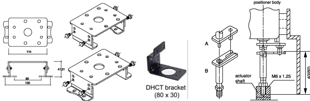
Multi-size bracket
