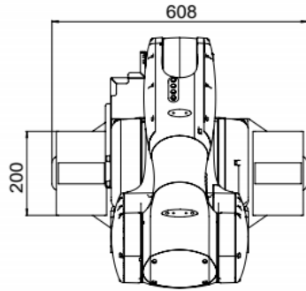
(c) 俯视图
