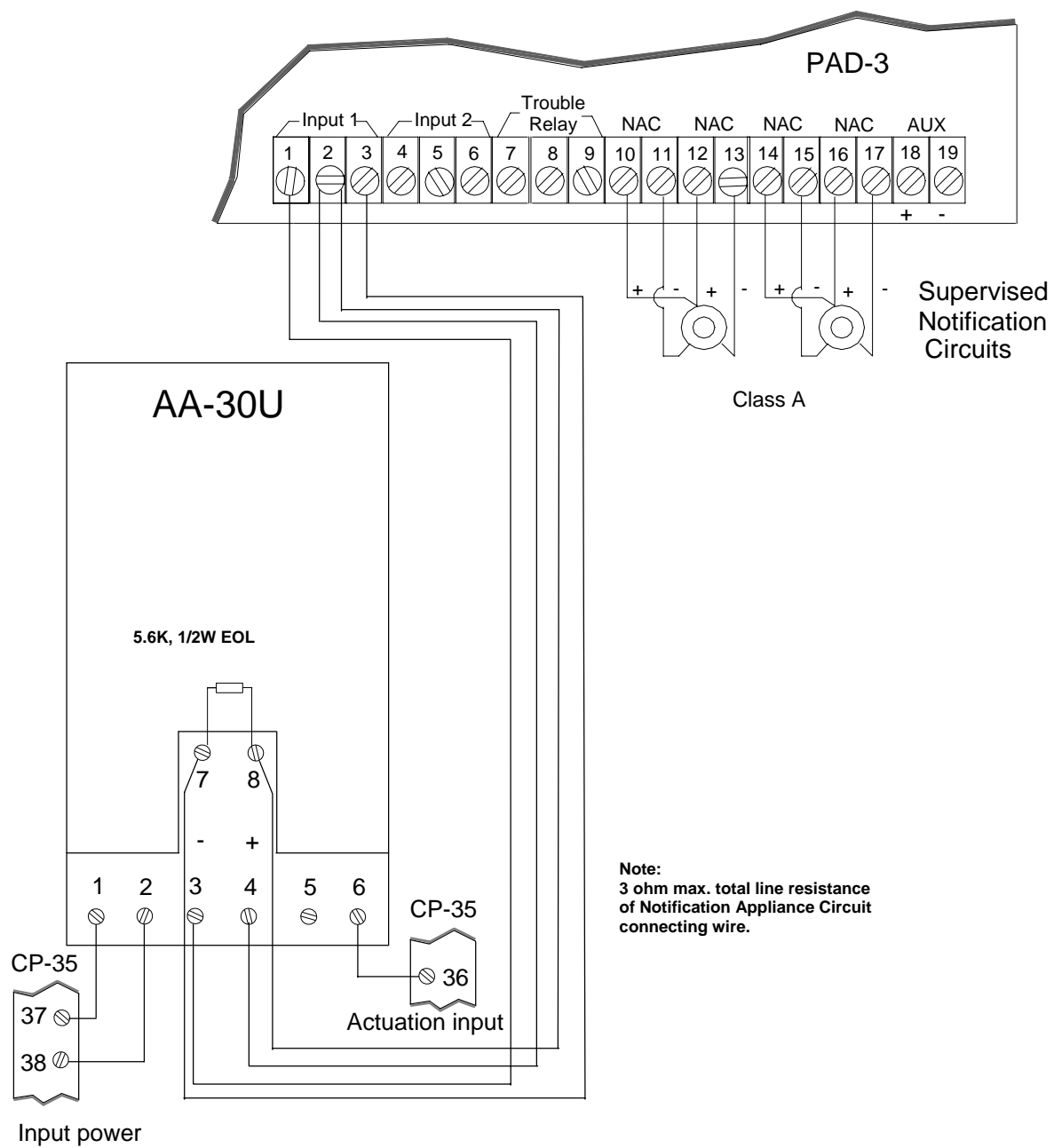
Figure 3-7. Connection to AA-30U
