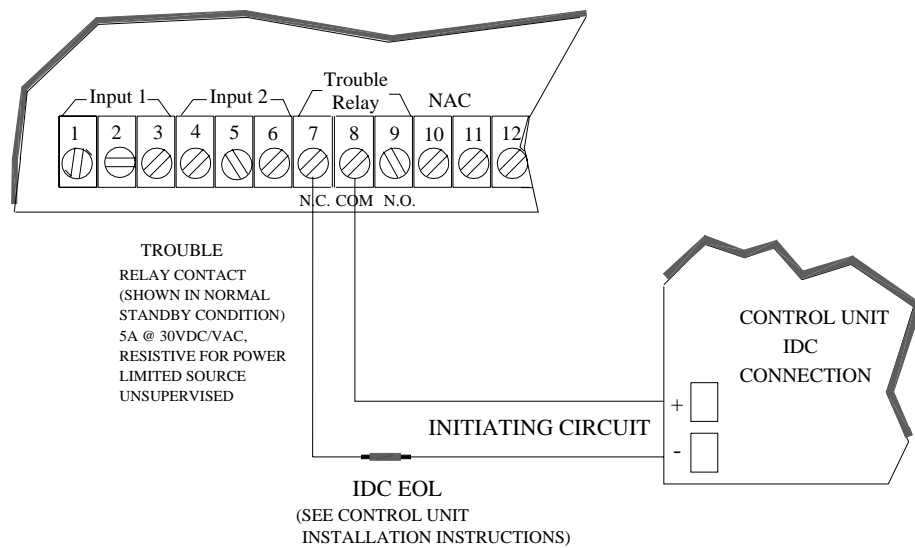
Figure 2-11. Trouble Relay Connection Example
