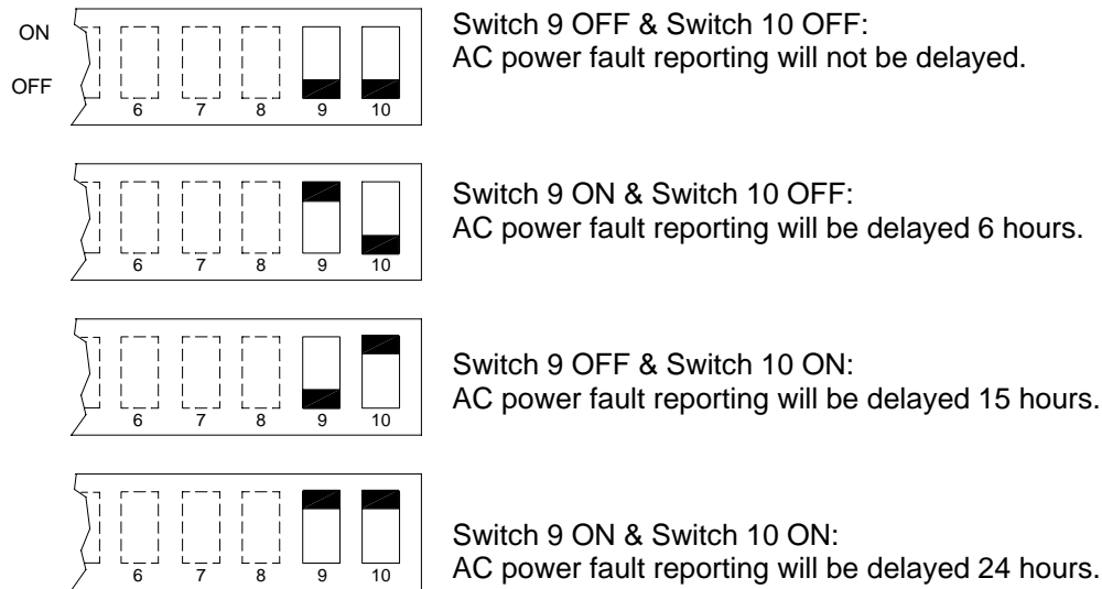
Figure 5-5. Setting DIP Switch 9 and 10
