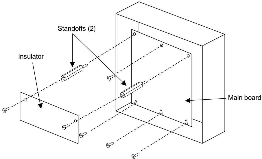
Figure 2-1. Mounting the PAD-3-MB
