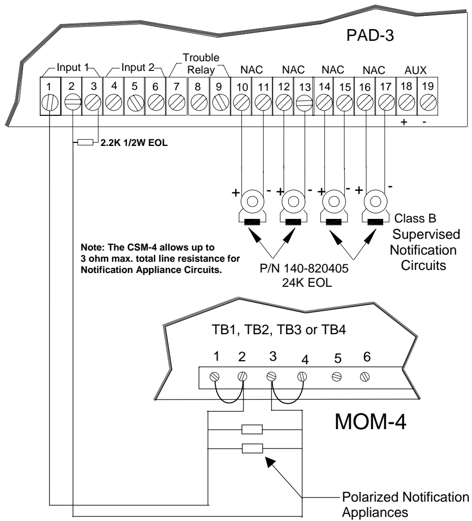
Figure 3-2. Connection to CSM-4
