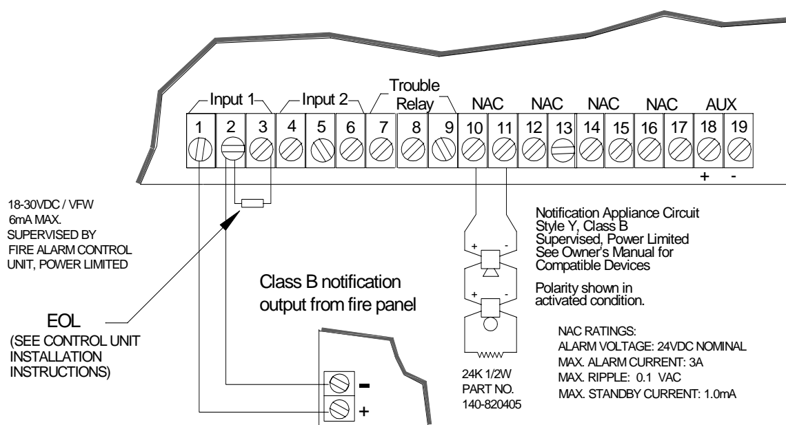
Figure 2-8. Style Y (Class B) Supervised Input/Output Connections
