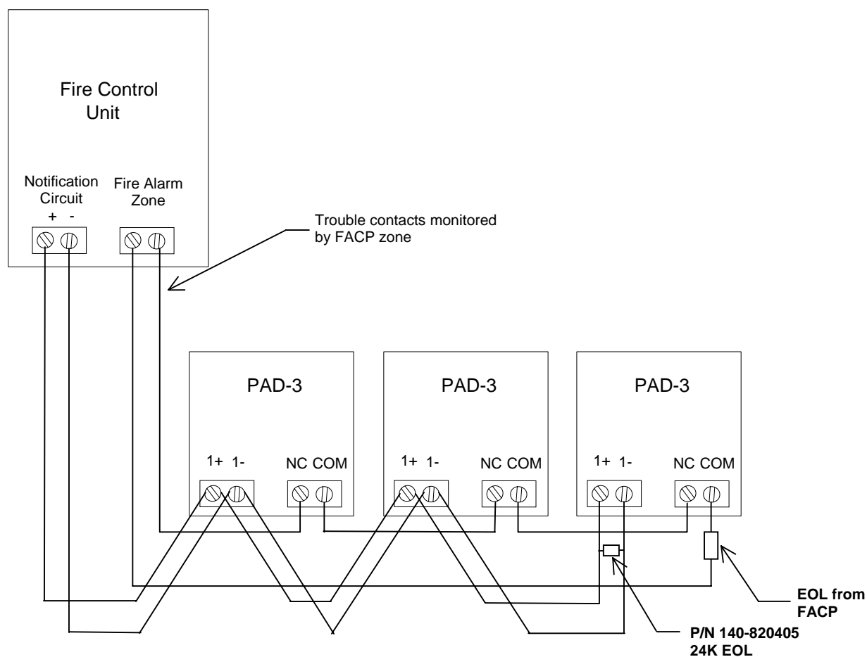
Figure 4-7. Multiple PAD-3s activated by a single notification circuit
