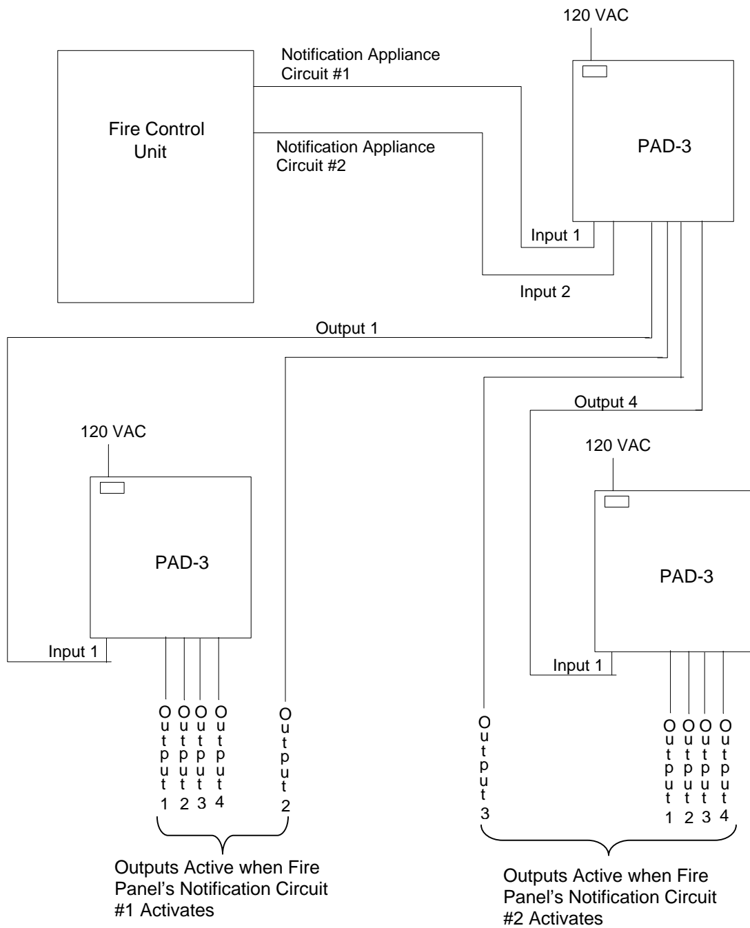
Figure 4-6. Each control signal circuit activates five output circuits
