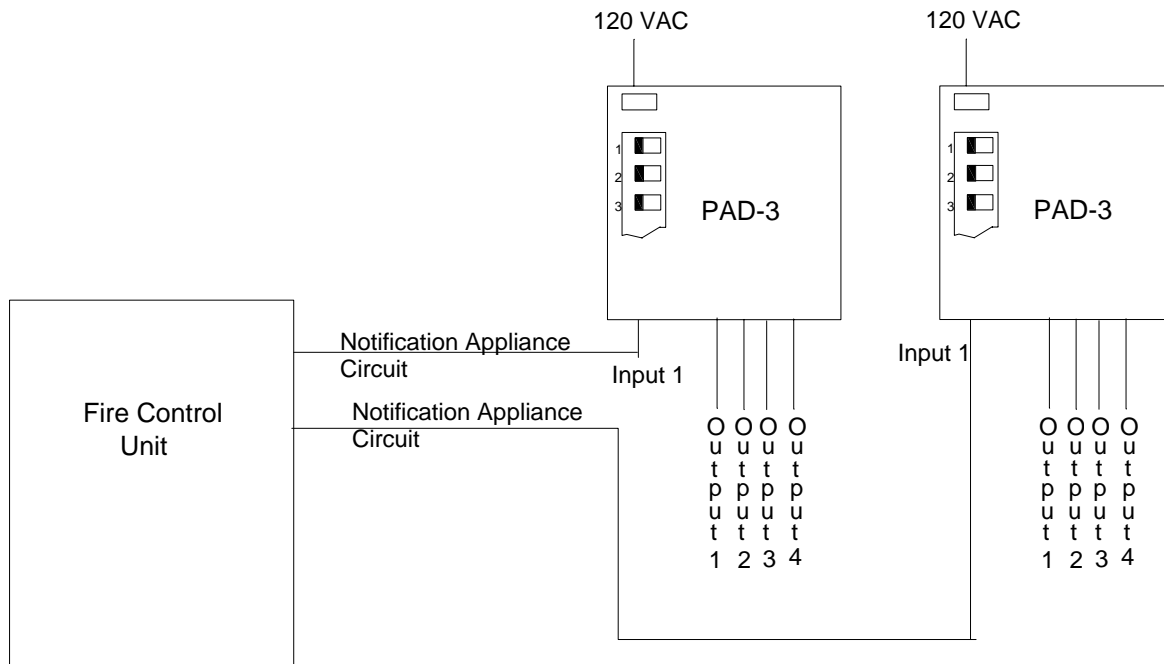
Figure 4-4. One Control Panel activating two PAD-3s
