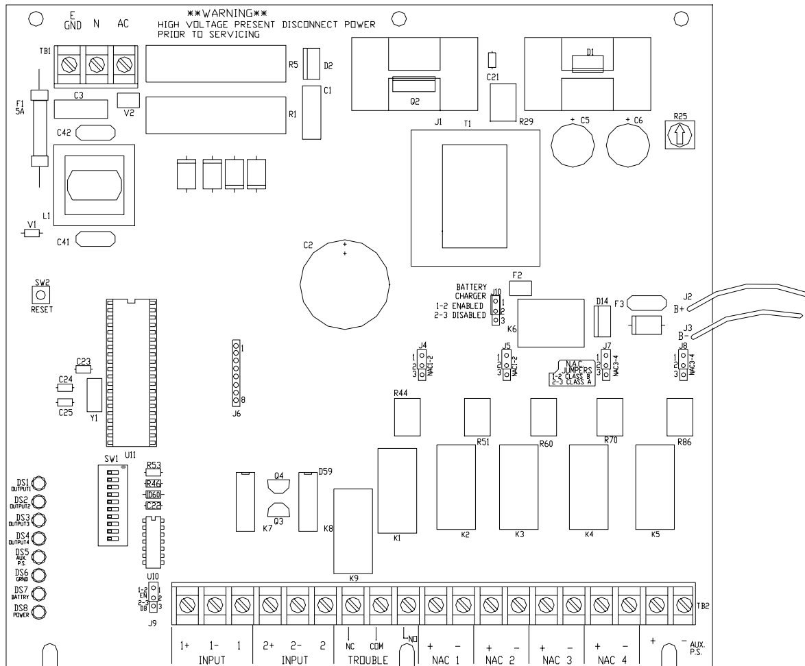
Figure 2-2. PAD-3 PC Board Layout
