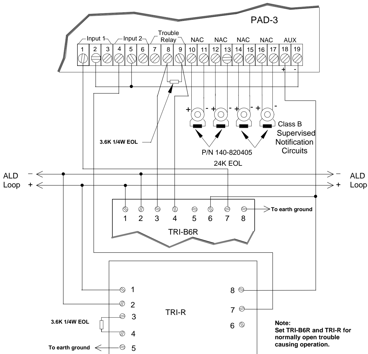
Figure 3-9. Connection to TRI-B6R and TRI-R
