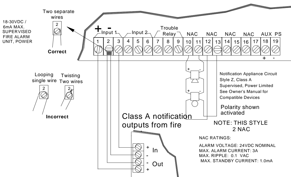
Figure 2-9 Style Z (Class A) Supervised Input/Output Connections
