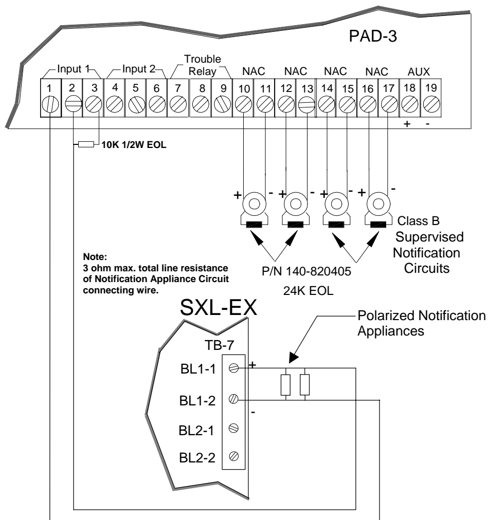
Figure 3-4. Connection to SXL-EX
