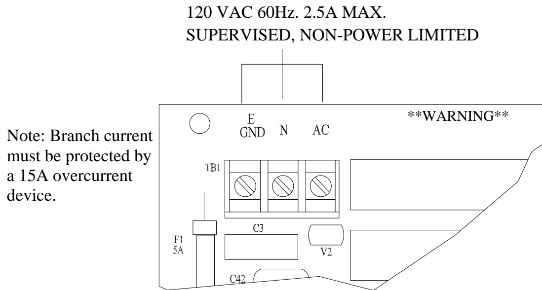
Figure 2-3. AC Wiring
