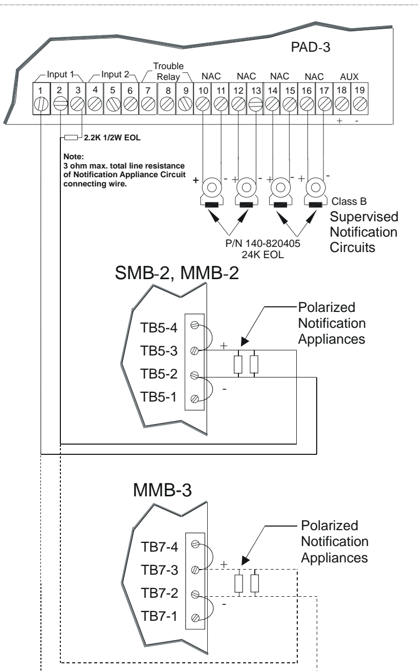
Figure 3-1. Connection to MXL, MXL-IQ
