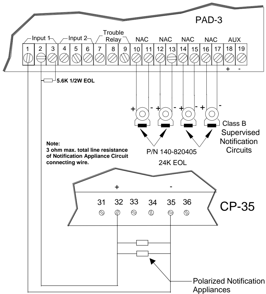
Figure 3-5. Connection to CP-35
