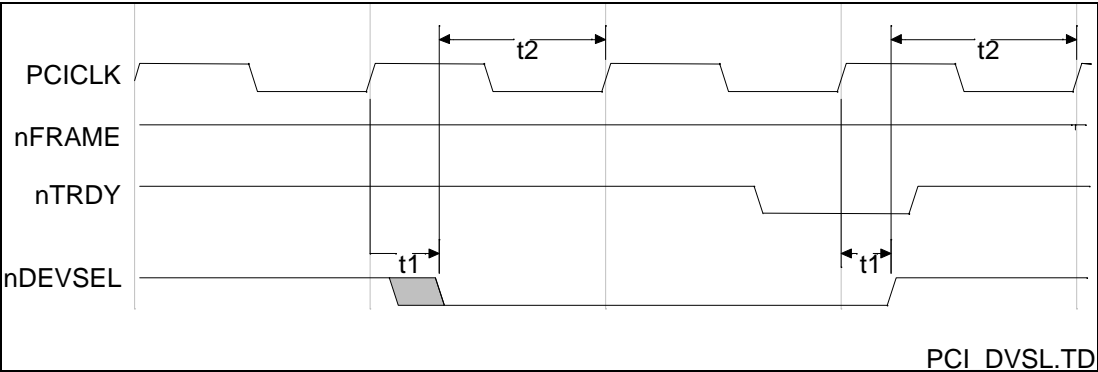
FIGURE 7 - PCI/nDEVSEL TIMING
