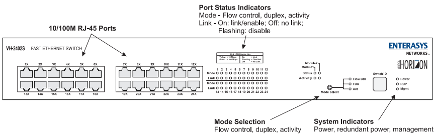
Figure 1-1. VH-2402S Front Panel
