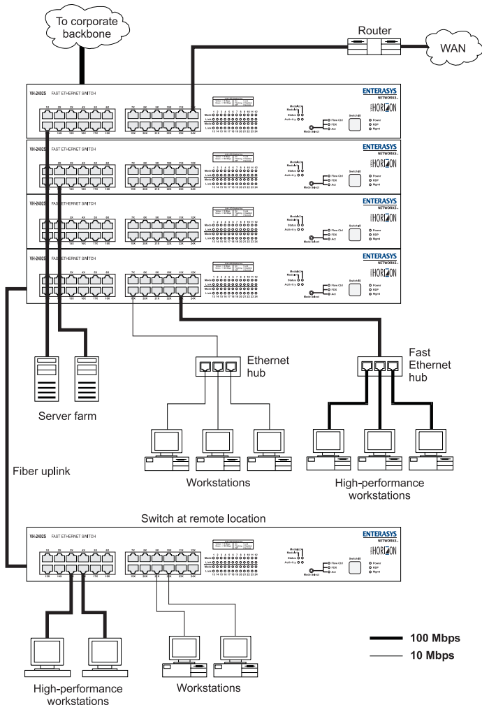
Figure 1-5. Local Backbone Application
