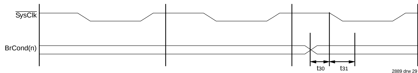
Figure 21. Direct Branch Condition Input Timing
