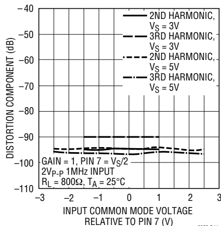
Distortion vs Input Common Mode
