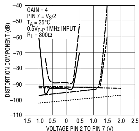
Distortion vs Output Common Mode
