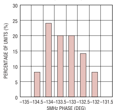
5MHz Phase Distribution (50 Units)
