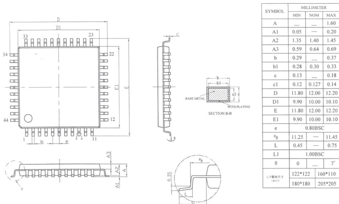
Figure 24-2 LQFP44 封装尺寸
