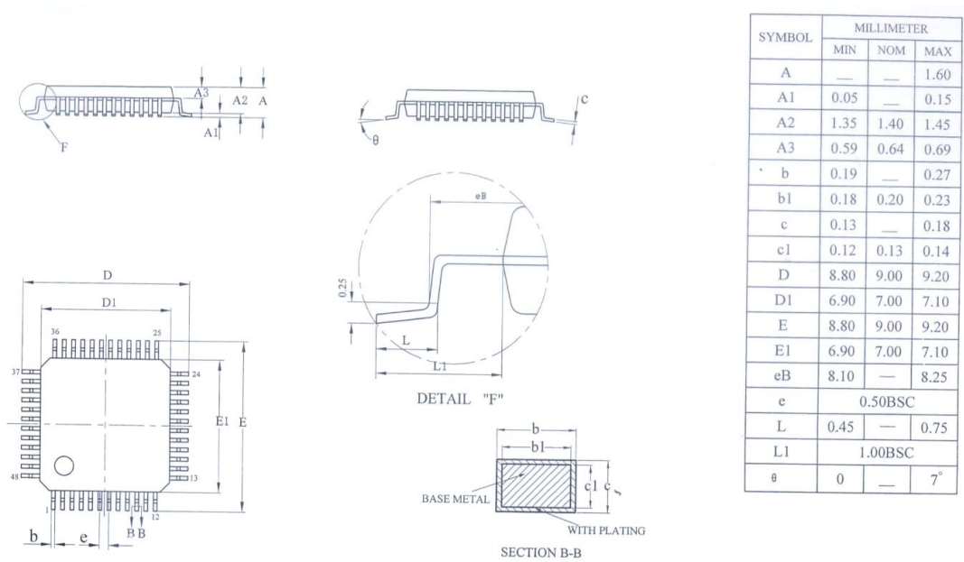
Figure 24-1 LQFP48 封装尺寸
