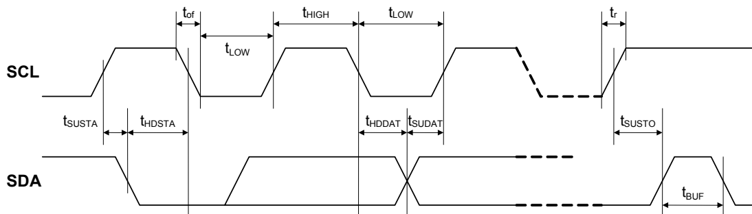
Figure 2. I 2 C Timing Parameters
