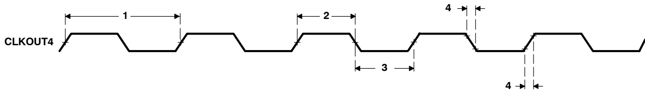
Figure 7-2. CLKOUT4 Timing
