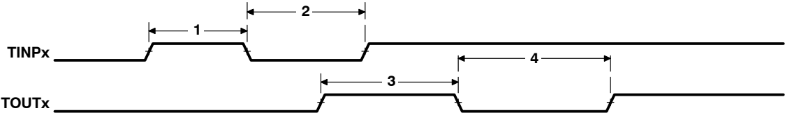
Figure 7–42. Timer Timing
