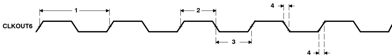
Figure 7-3. CLKOUT6 Timing
