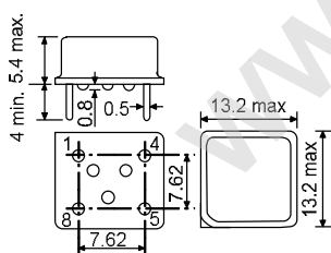
Figure 1) ECS-2100 Series - Side, Bottom and Top views
