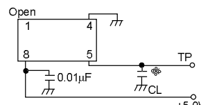
Figure 5) HCMOS Measurement Circuit ( C_L = 15 pF)
