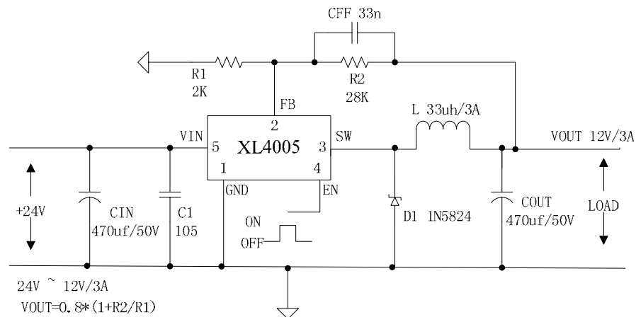
Figure6. XL4005 System Parameters Test Circuit (24V ~ 12V/3A)
