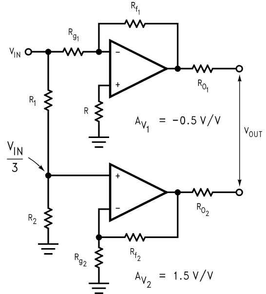
FIGURE 3. Single-to-Differential Line Driver
