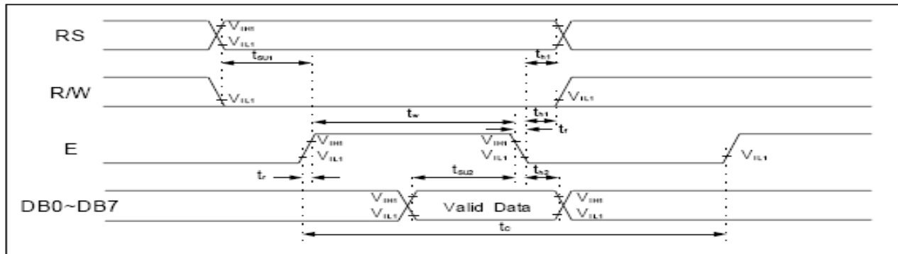
Figure 6 . Write Mode Timing Diagram
