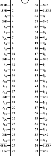
Pin Assignment for SSOP
