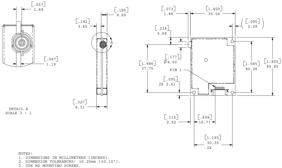
Figure 4. GPS 15H-F & 15L-F Dimensions
