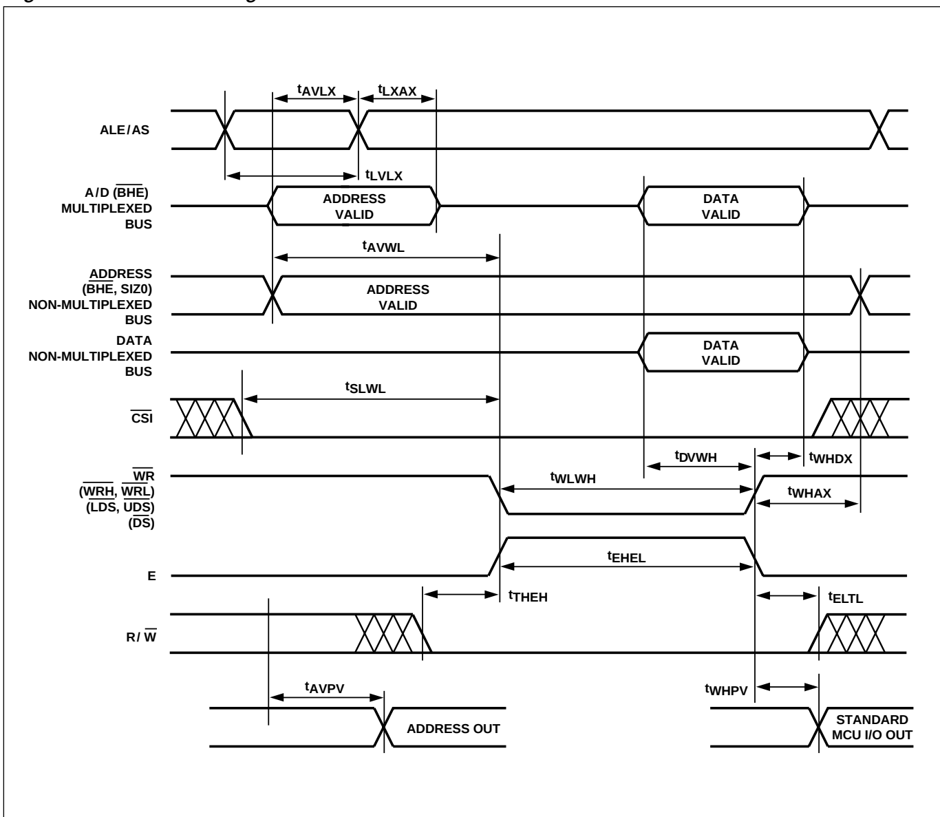
Figure 53. Write Timing
