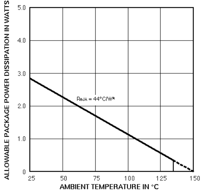
A3940KLW (SOIC)
