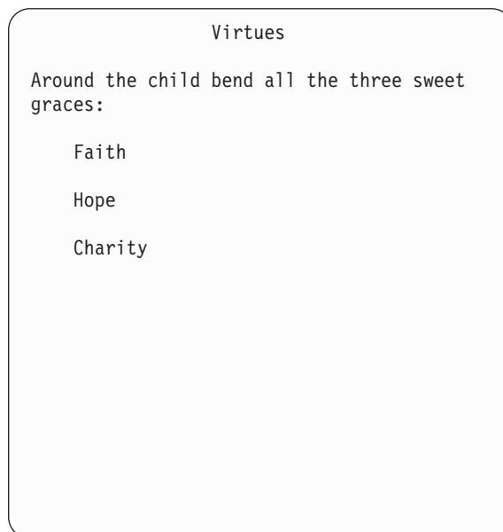
Figure 50. Simple list
