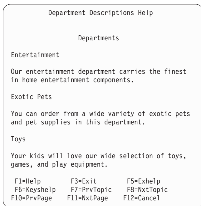
Figure 124. Headings
