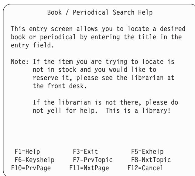
Figure 141. NT
