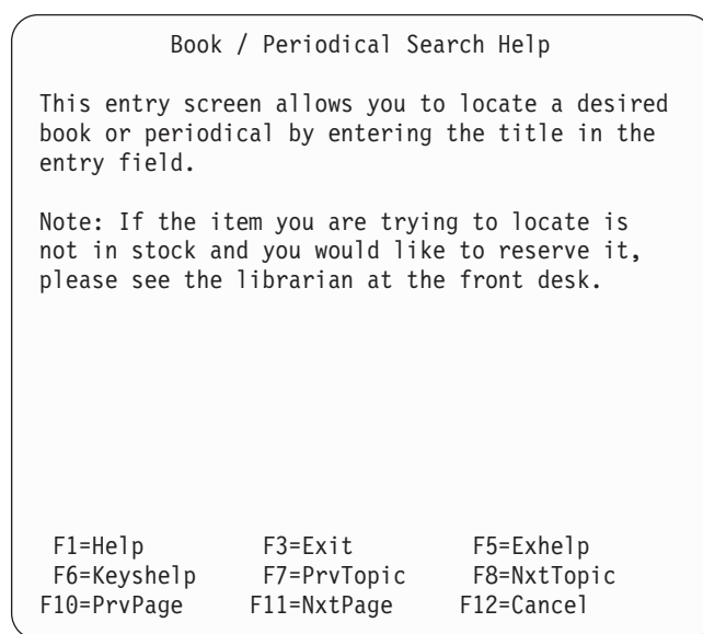
Figure 139. Note
