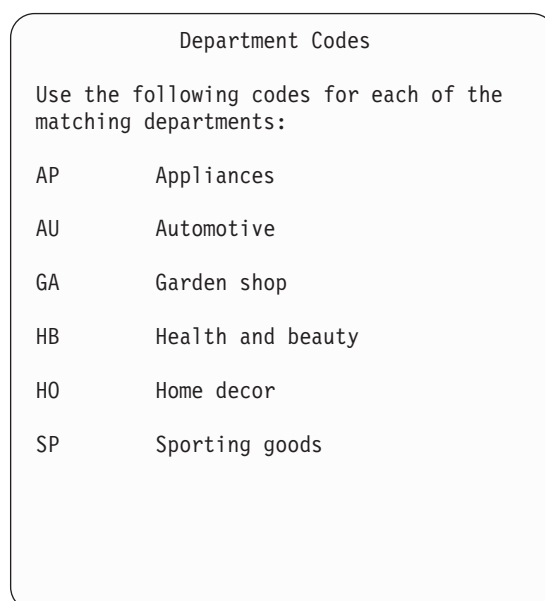
Figure 56. Definition list
