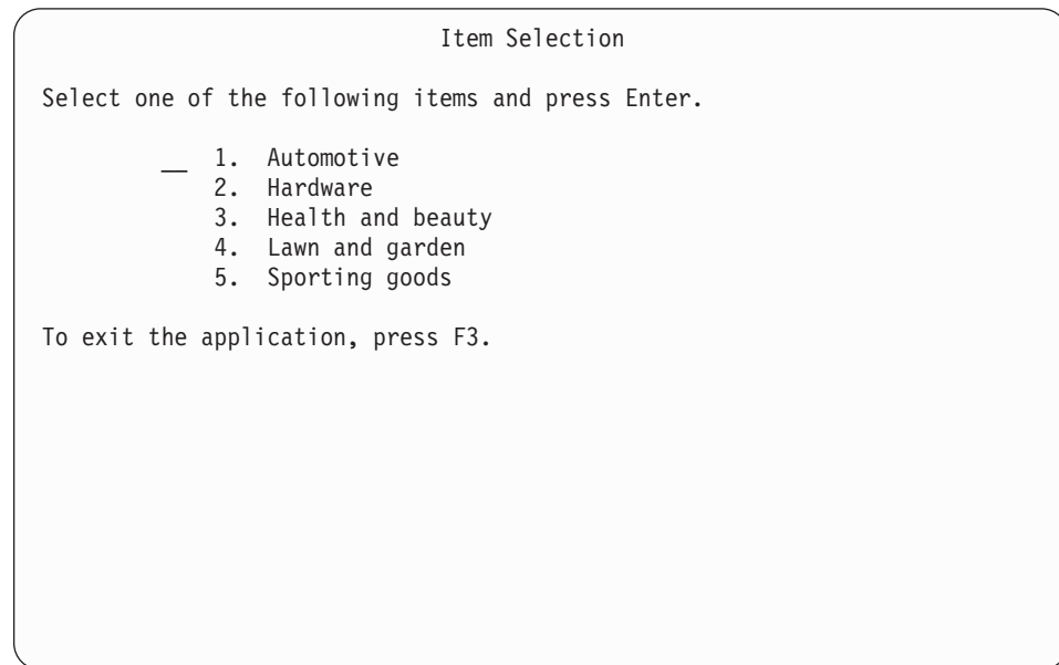
Figure 14. AREA MARGINW=10
