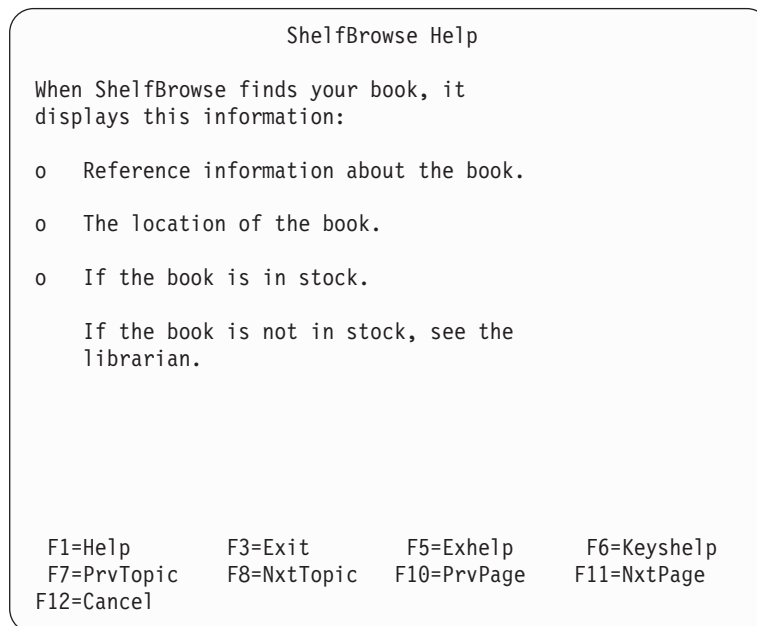
Figure 126. Information region
