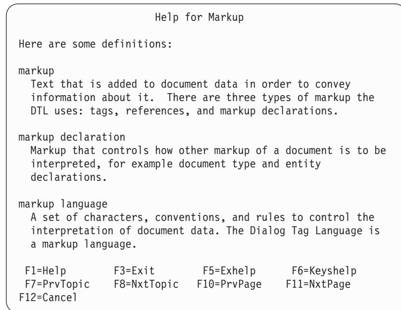
Figure 108. Definition Terms
