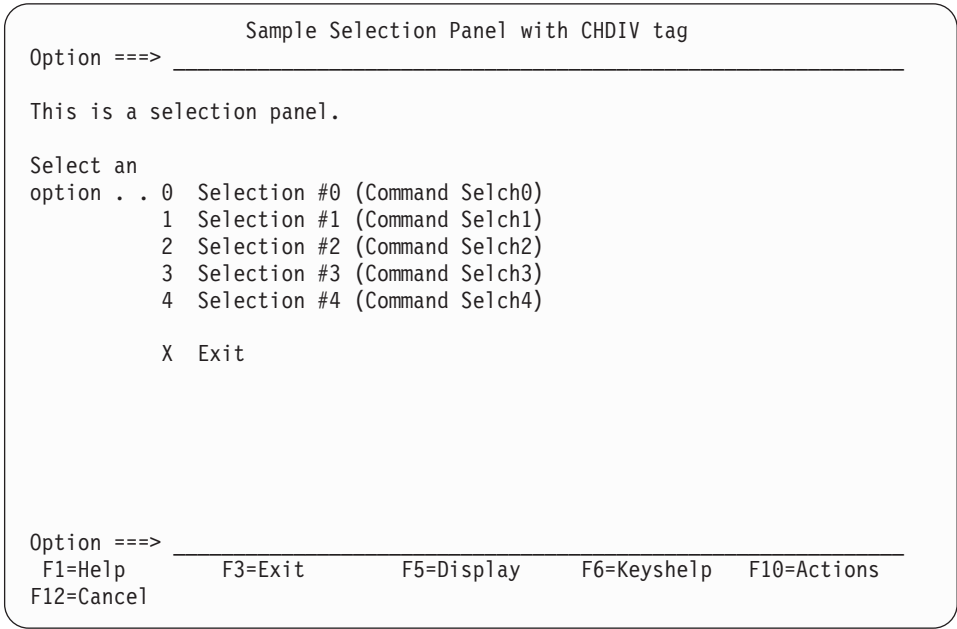
Figure 95. Choice divider
