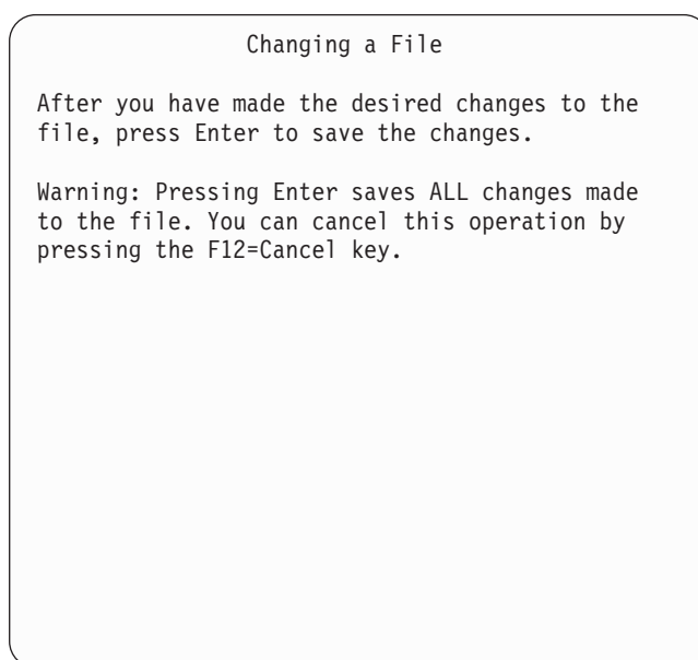
Figure 66. Warning
