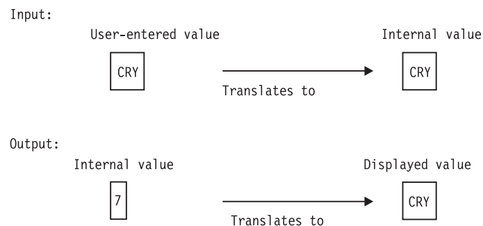
Figure 27. Variable translation
