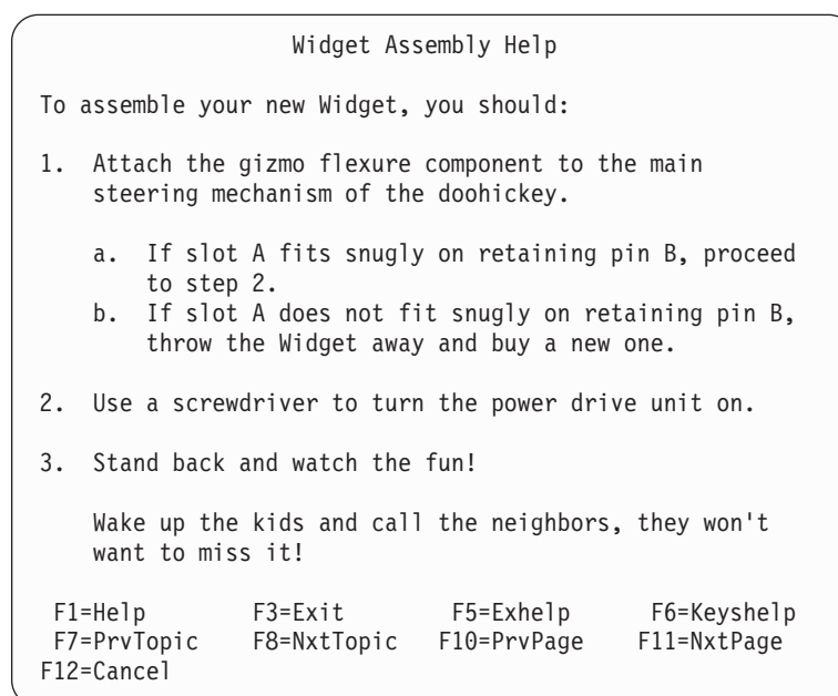
Figure 142. Ordered lists
