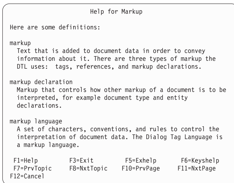
Figure 101. Definition descriptions
