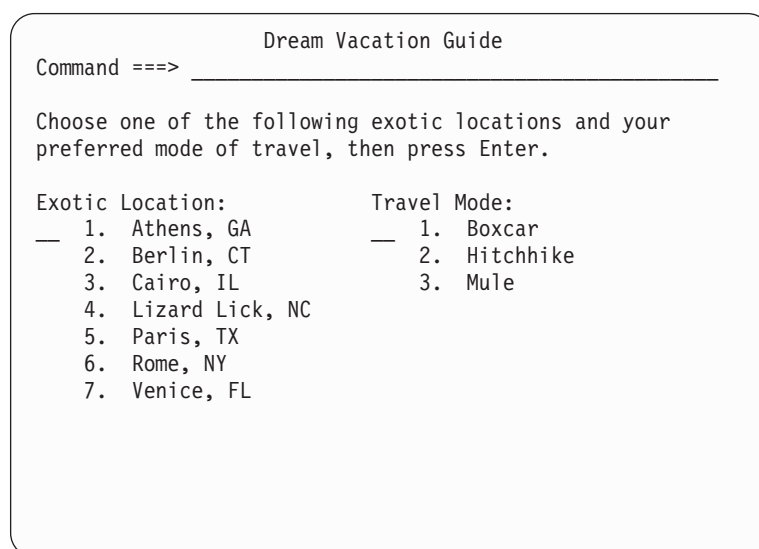
Figure 150. Panel instructions
