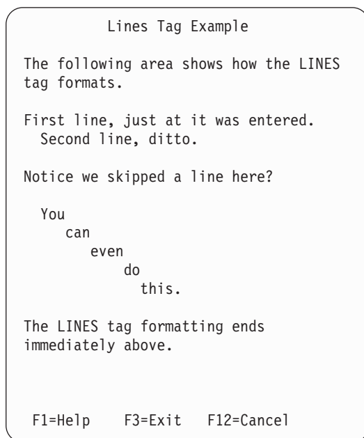
Figure 130. LINES
