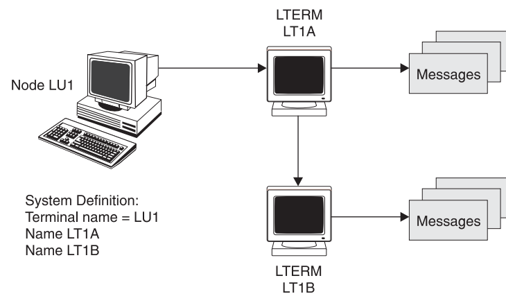
Figure 21. Static Resources
