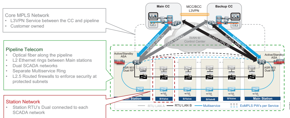
Figure 4-1 Operational Telecoms Network
