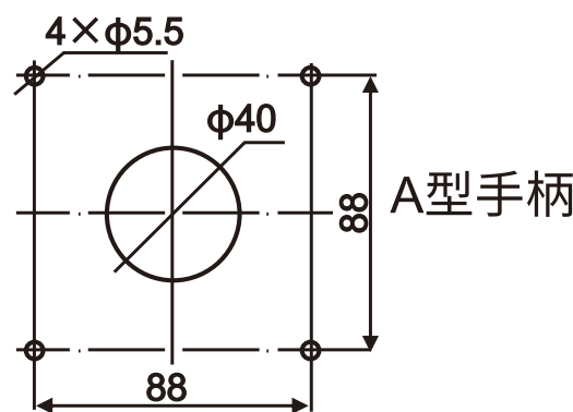
柜外通用手柄800A~3200A
