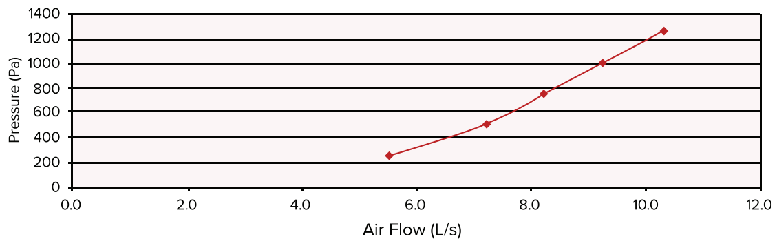
Performance Data
