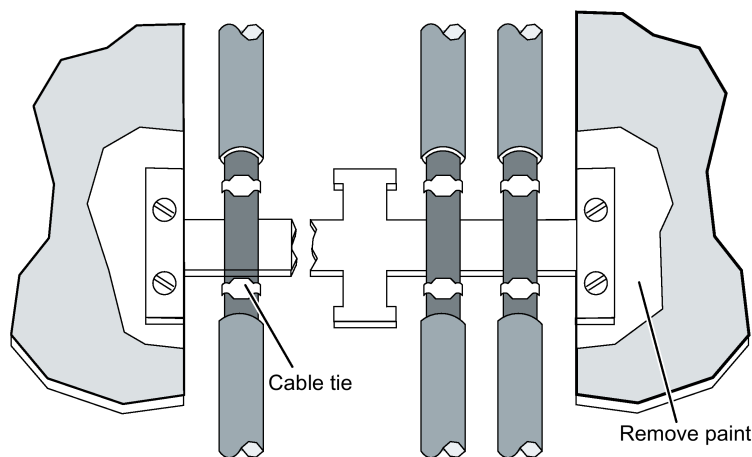
Figure 6-6 Connection of shielding bus
