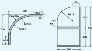
External Curved Door to Suit 300x300 Unit
