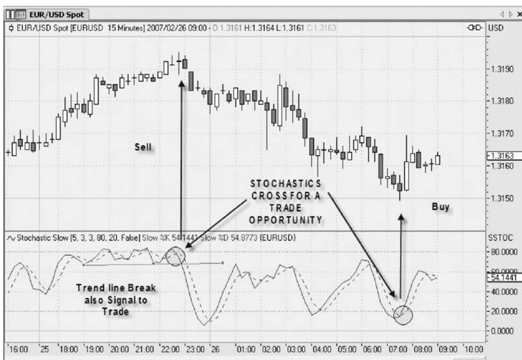
FIGURE 12.11 Stochastic Crossover.
