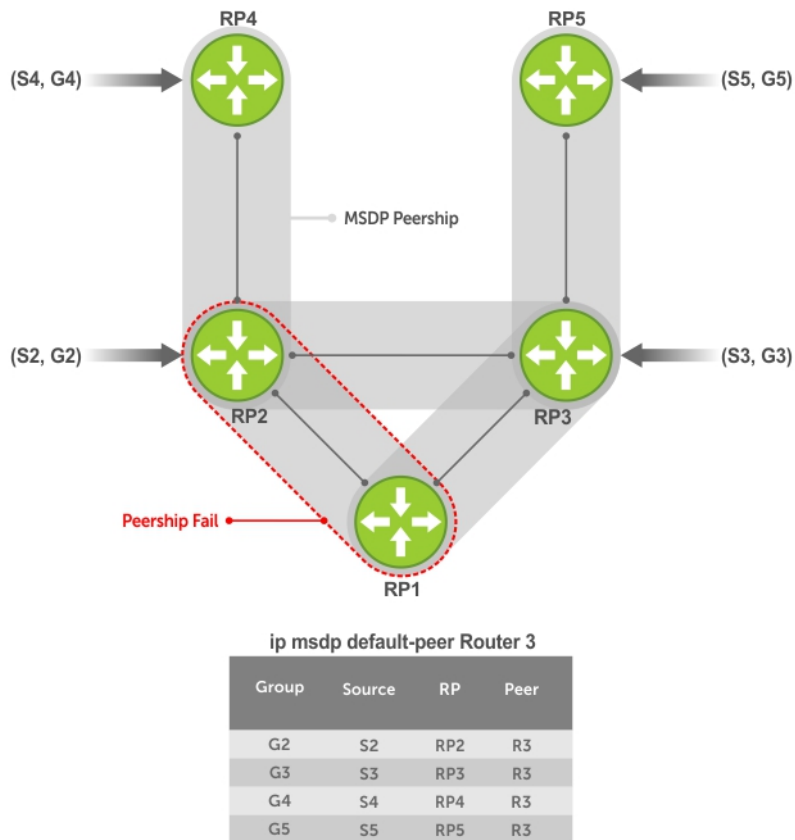
Figure 93. MSDP Default Peer, Scenario 3
