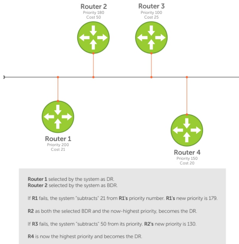
Figure 103. Priority and Cost Examples
